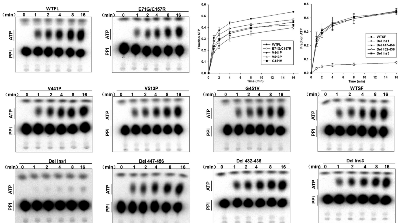
FIGURE 5. PPI-exchange activity of WT and mutants of hGlyRS. The reactions were carried out using 100 nM enzymes. Formation of enzyme-bound aminoacyl-adenylate intermediate allows conversion of PPI into ATP. The reactions were quenched at different time points (0, 1, 2, 4, 8, and 16 min), separated on cellulose polyethyleneimine TLC plate, and visualized by a phosphorimaging plate. As shown in the top right corner , the insertion 3 point mutations or deletions did not greatly affect PPI exchange activities, when compared with the WT.
