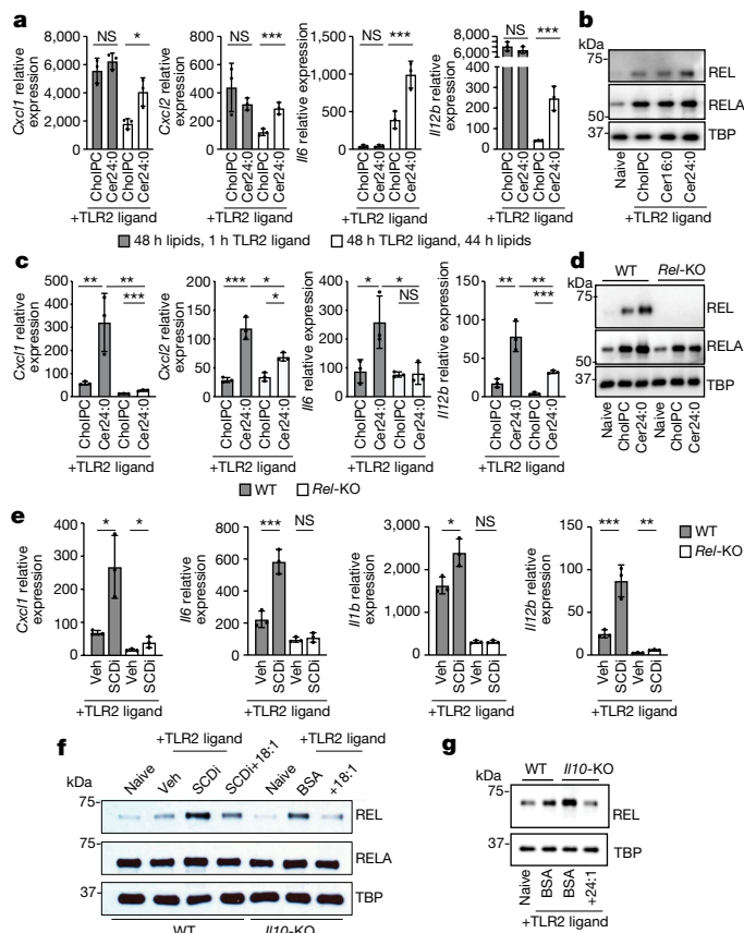
Fig. 4 | REL is required for ceramide-mediated induction of inflammatory gene expression. a , qPCR analysis of inflammatory gene expression in BMDMs pretreated with 30 \mu M Cer24:0 for 48 h, followed by 1 h activation with TLR2 ligand (50 ng ml -1 Pam3CSK4) versus 48 h TLR2 activation with 44 h 30 \mu M Cer24:0 treatment ( n = 3 ). b , Western blot analysis of RELA, REL and TBP (loading control) from nuclear extracts from naive or 48 h TLR2-activated wild-type peritoneal macrophages plus cholPC (vehicle), Cer16:0, or Cer24:0 for the last 44 h of the activation. Representative of three individual experiments. c , qPCR analysis of inflammatory gene expression in 48 h TLR2-activated wild-type or Rel -KO BMDMs plus cholPC (vehicle) or 30 \mu M Cer24:0 for the last 44 h of activation ( n = 3 ). d , Western blot analysis of RELA, REL and TBP (loading control) from nuclear extracts from naive or 48 h TLR2-activated wild-type or Rel -KO BMDMs plus cholPC (vehicle) or 30 \mu M Cer24:0 for the last 44 h of activation. RELA was blotted in parallel with REL and TBP. Representative of two individual experiments. e , qPCR analysis of inflammatory gene expression in 48 h TLR2-activated wild-type or Rel -KO BMDMs with or without 10 nM SCDi (Cay10566) for the last 44 h of activation ( n = 3 ). Veh, vehicle. f , Western blot analysis of REL, RELA and TBP (loading control) in nuclear extracts from naive or 48 h TLR2-activated wild-type or Il10 -KO BMDMs plus SCDi, BSA or 25 \mu M BSA-18:1 for the last 44 h of the activation. Representative of three individual experiments. g , Western blot analysis of nuclear extracts from naive or 48 h TLR2-activated wild-type or Il10rb -KO BMDMs plus BSA or 25 \mu M BSA-24:1 for the last 44 h of the activation for RELA, REL and TBP (loading control). Representative of two experiments. All experiments are reported as mean of biological replicates \pm s.d. * P < 0.05 , ** P < 0.01 , *** P < 0.005 (two-tailed unpaired Student's t -test).
