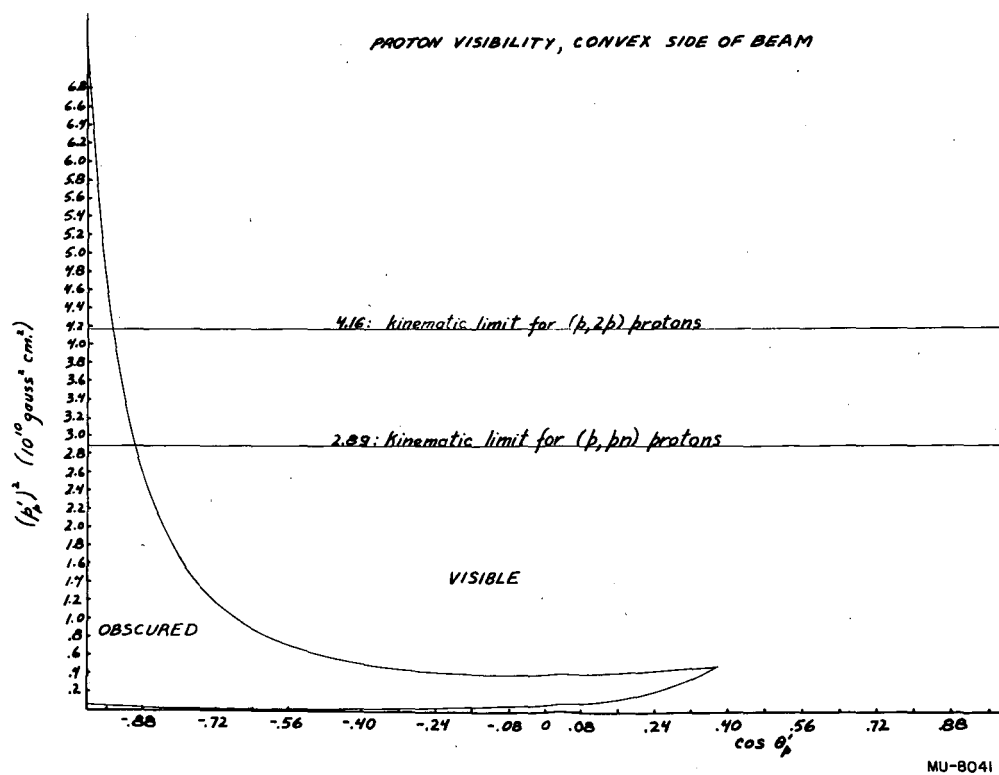
Fig. 22a Momentum Space Available to Protons.
