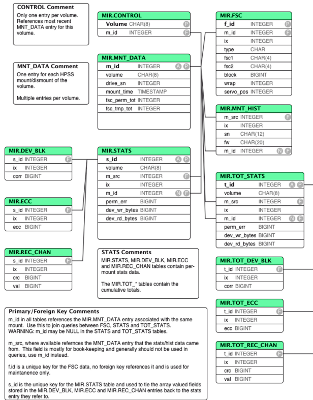
Fig. 2. Database Schema for MIR Statistics
