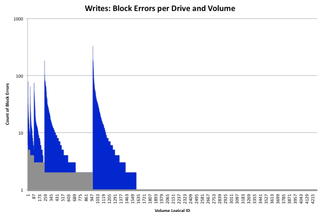
Fig. 3. Block Write Errors
