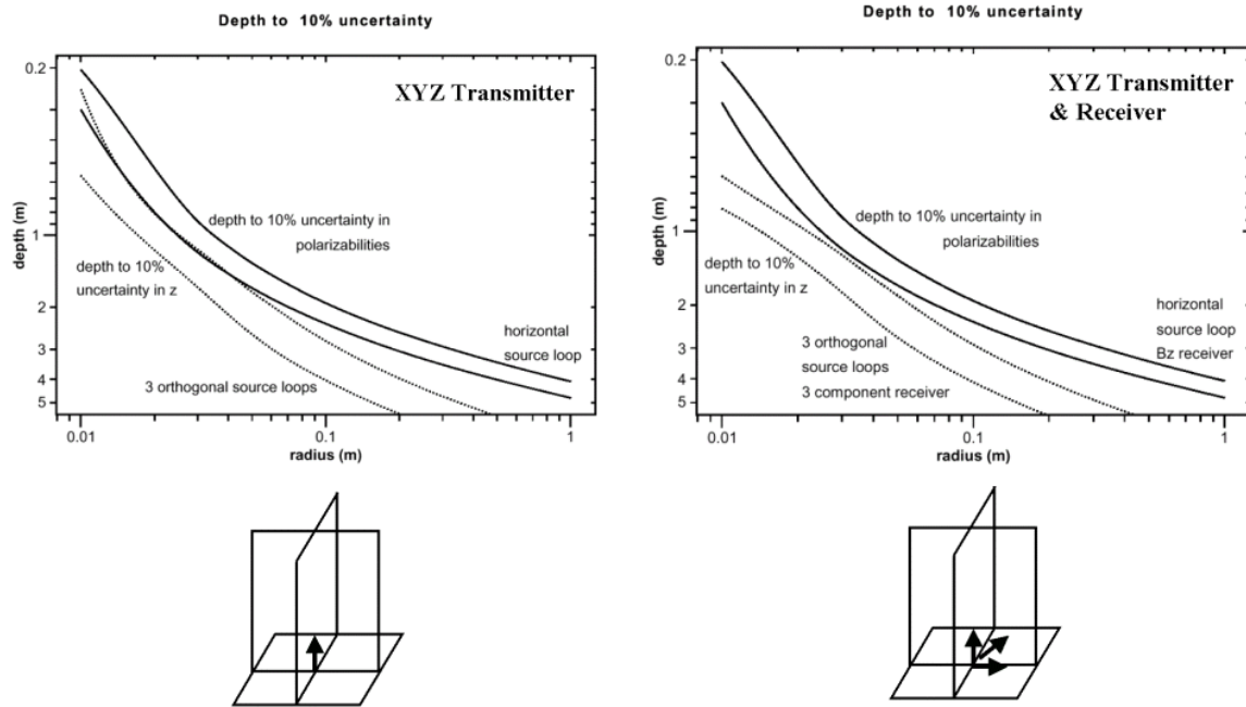
Figure 1: Depth to 10% polarizability uncertainty and 10% uncertainty in depth as a function of sphere radius for TxTyTz-Bz and TxTyTz – BxByBz systems.
