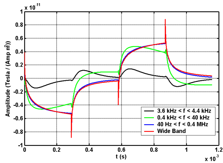
Figure 3. Effect of system bandwidth on the observable target signal.
