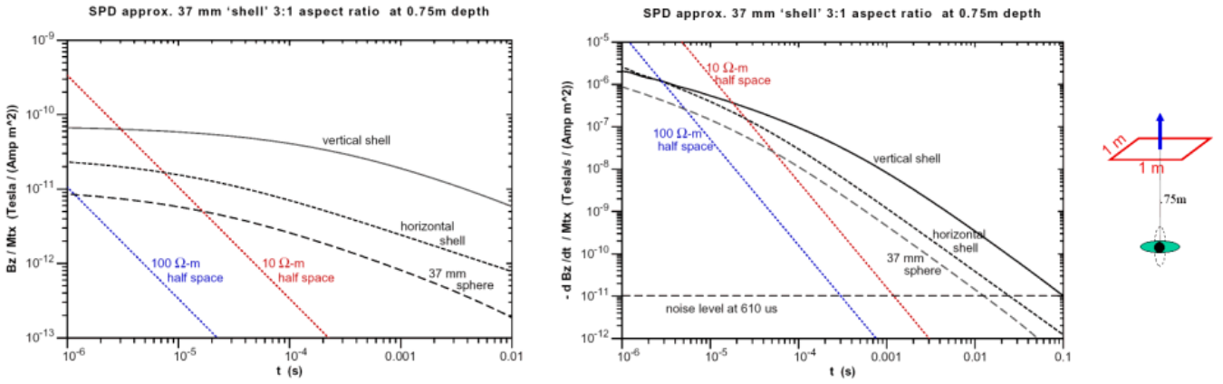
Figure 2: Amplitude of B and dB/dt response for 37 mm sphere, horizontal and vertical shells 3:1 aspect ratio at the depth of 0.75 m as a function of time together with responses for 10 \Omega -m and 100 \Omega -m half-space.
