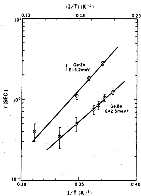
Figure 35 Time constant of the slow component as a function of inverse temperature
