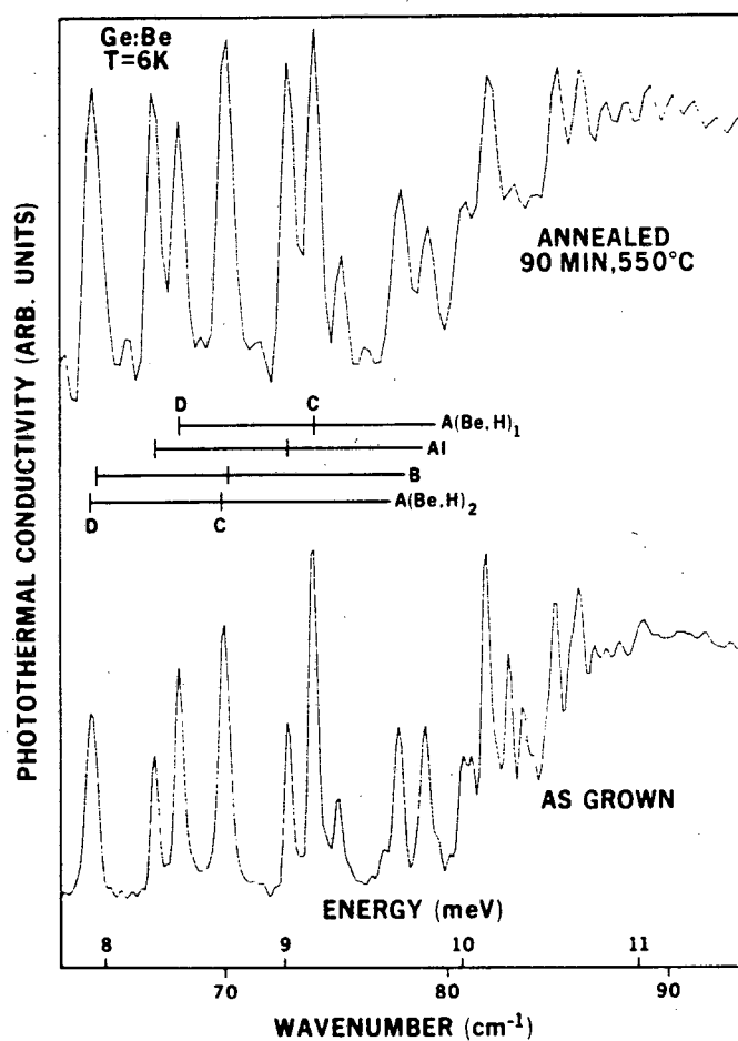
Figure 21 PTIS spectra at T = 6 K
