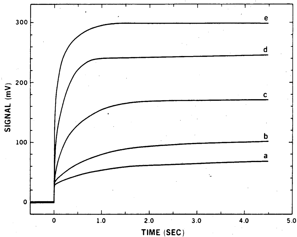
Figure 34 Compiled data from Figure 33 showing the effect of increasing temperature on signal size
