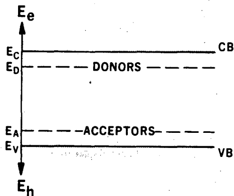
Figure 3 Single level photoconductor band diagram
