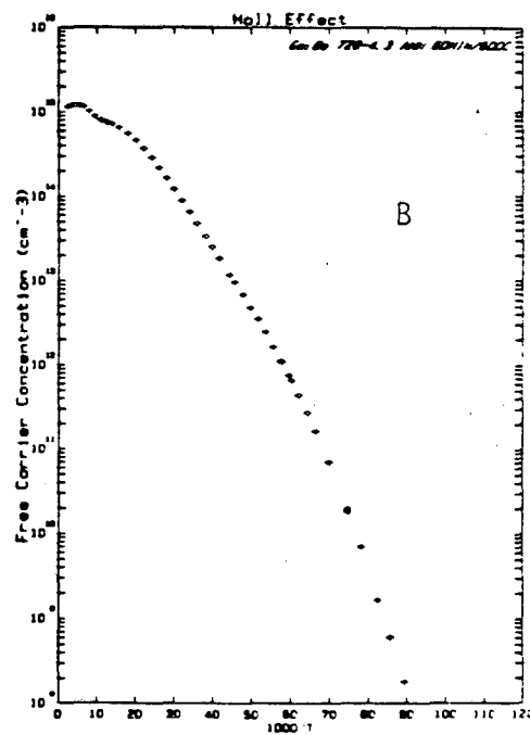
Figure 10 Freeze-out curves for A) N_{A_S} > N_D and B) N_{A_S} < N_D
