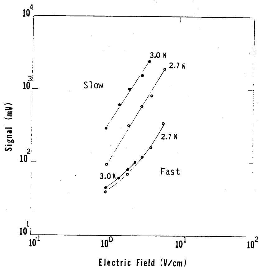
Figure 39 Amplitude of fast and slow component as a function of bias
