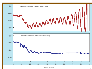
Near bottom left: Comparison of predicted conditions prior to August 10, 1996 blackout (lower panel) and conditions actually recorded by phasor technologies (upper panel) showed that the planning models were not able to accurately capture underlying causes of the blackout.
