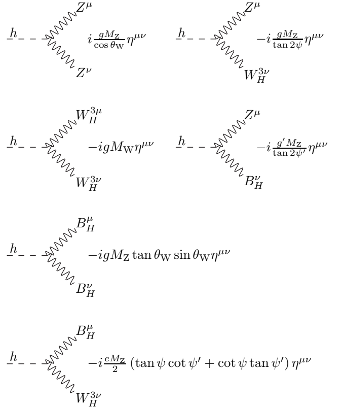
FIG. 1. Cubic couplings between the physical Higgs boson h and pairs of neutral gauge bosons.
