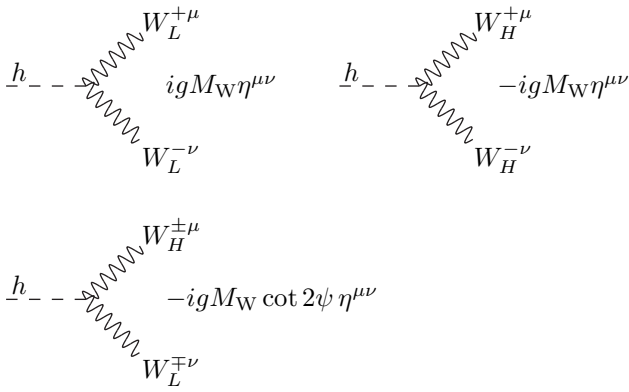
FIG. 2. Cubic couplings between the physical Higgs boson h and pairs of charged gauge bosons.
