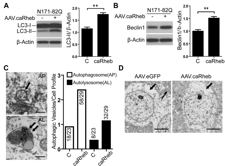
Figure 4. AAV.caRheb increases basal autophagy in N171-82Q mice (A and B) Biochemical assessment of autophagy (LC3 and Beclin1) in striatal lysates from N171-82Q mice after unilateral injection of AAV.caRheb at 7 weeks of age. Striata were harvested 3 weeks post-injection. Uninjected contralateral striata serve as internal controls (N=6 mice per group). Representative western blots and densitometry analysis revealed increased LC3II and Beclin1 levels in AAV.caRheb-treated N171-82Q mice striata. \beta -actin was used as a loading control. Data are mean \pm SEM. **P < 0.01 ; Student's t-test. (C) Left panels: representative photomicrographs of an autophagosome (arrow) and an autolysosome (double arrow). Scale bar is 0.5 \mu m. Right panel: frequency of autophagosomes and autolysosomes detected in striatal neurons from AAV.eGFP and AAV.caRheb treated N171-82Q mice (3 mice examined per group; 7-10 cells/hemisphere/animal). Ratio indicates number of autophagosome or autolysosome over total number of cells counted. (D) Ultrastructural TEM analysis of striatal sections from N171-82Q mice after AAV.eGFP or AAV.caRheb injections into opposite hemispheres (N=3 mice per group). Left panel: a representative photomicrograph of striatal neurons from control treated striata shows electron-lucent cytoplasm, devoid of endoplasm granular mass and organelles. Right panel: AAV.caRheb treated neurons show normal cytoplasm enriched with organelles and endoplasm granular mass. Scale bar is 5 \mu m.
