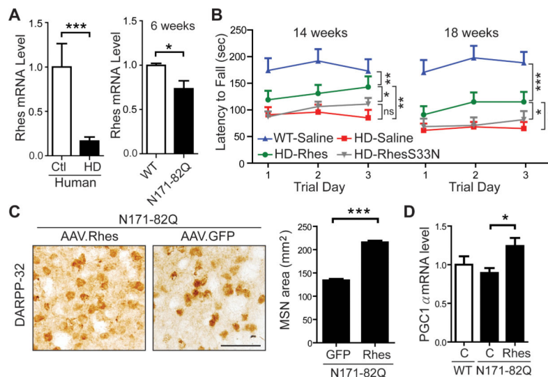
Figure 7. Intrastriatal Rhes overexpression improves disease phenotypes in N171-82Q mice (A) RT-qPCR analysis of endogenous Rhes levels from striatal lysates of unaffected individuals (Ctl, N=4) and HD patients (N=10), and 6-week-old N171-82Q (N=5) and WT (N=4) littermates. Data represent mean \pm SEM. * P <0.05, *** P <0.001, Student's t-test. (B) Rotarod assessment of N171-82Q and WT mice after bilateral injection of AAV.Rhes, AAV.RhesS33N, or saline into the striatum at 7 weeks of age (N=10-14 mice per group at 14 weeks of age; N=6-13 mice per group at 18 weeks of age). Rotarod data from three consecutive days at 14 and 18 weeks of age are shown as latency to fall. Saline and AAV.RhesS33N-injected N171-82Q mice performed significantly worse compared to AAV.Rhes-injected N171-82Q mice on the rotarod at 14 and 18 weeks of age. NS=Not statistically significant. Data represent mean \pm SEM. * P <0.05; ** P <0.01; *** P <0.001, One-way ANOVA with Tukey's post-hoc test. (C) DARPP-32 staining and quantification of MSN area of N171-82Q mice striatal tissue sections after unilateral injection of AAV.Rhes and contralateral injection of AAV.GFP at 7 weeks of age. Tissues were harvested at 19 weeks of age (N=3 mice/group; GFP=245 cells; Rhes=251 cells). Data represent mean \pm SEM. *** P <0.001, Student's t-test. Scale bars: 50 \mu m. (D) qPCR analysis of PGC-1 \alpha in striata from AAV.Rhes- or saline-treated N171-82Q and WT mice (n=6-9 per group) harvested at the end of the study (19 weeks of age). C=Control. * P <0.05, Student's t-test.
