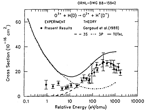
Fig. 2. Comparison of merged-beams data for O^{3+} + H(D) with theoretical calculations (Ref. 8) for capture into the 3s and 3p states.
