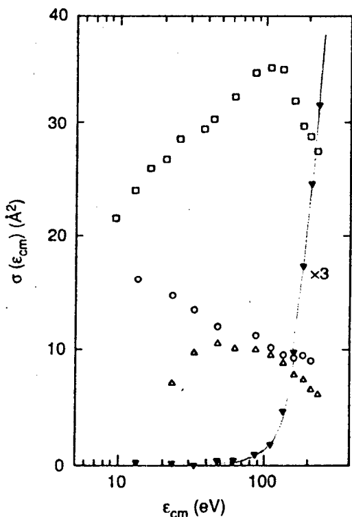
Fig. 2. - Cross sections for collisional detachment (▼), F^- production (□), SF_5^- production (○), and charge transfer (Δ) as a function of the relative collision energy. Note that the detachment data have been multiplied by a factor of three.
