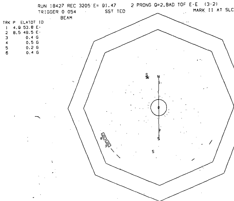
Fig. 19. Endcap e^+e^- event.
