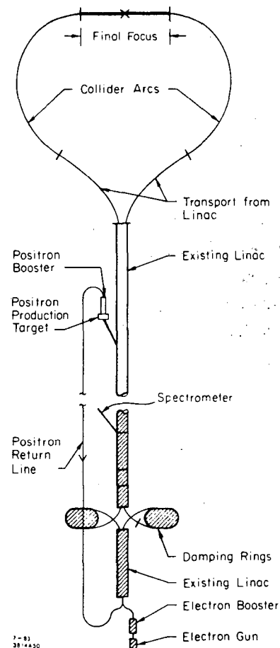
Fig. 1. Schematic layout of the SLC.
