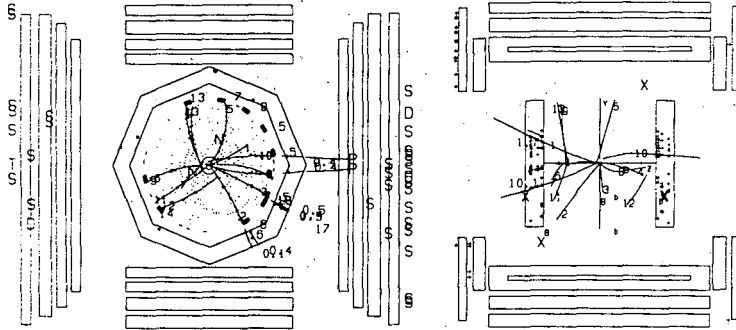
Fig. 18. Discarded event closest to passing the E_Z^{\min} cut.
