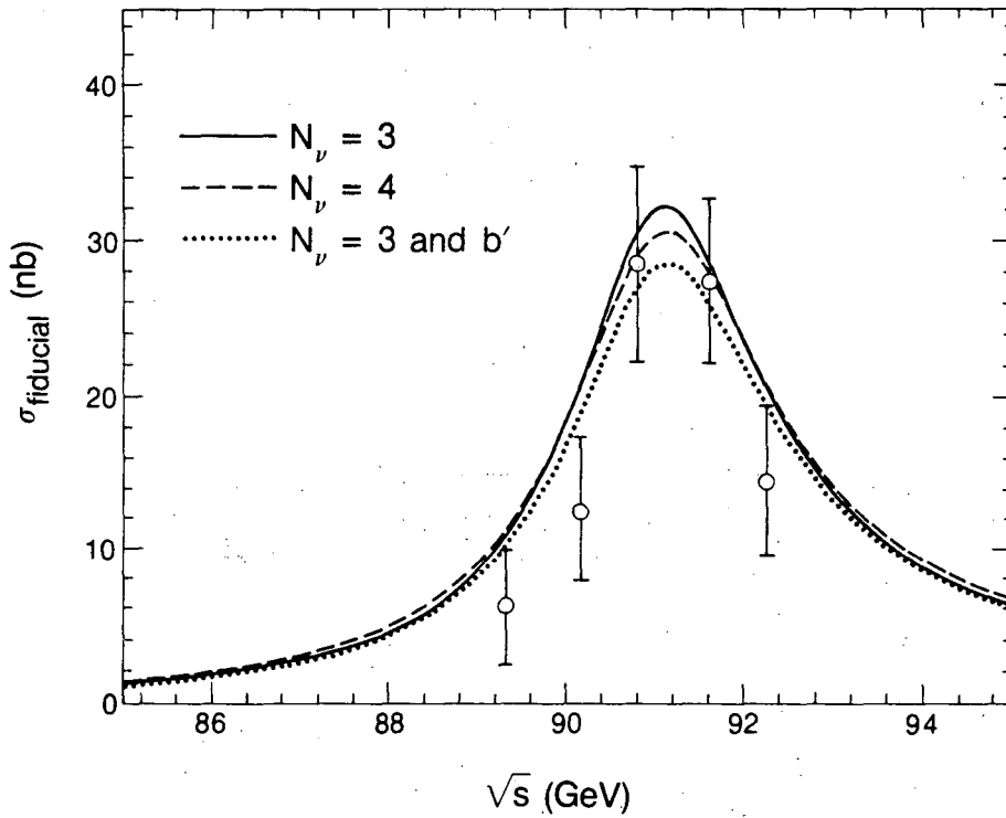
Fig. 23. Cross section for hadronic, \mu^+\mu^- and \tau^+\tau^- events as a function of center of mass energy.
