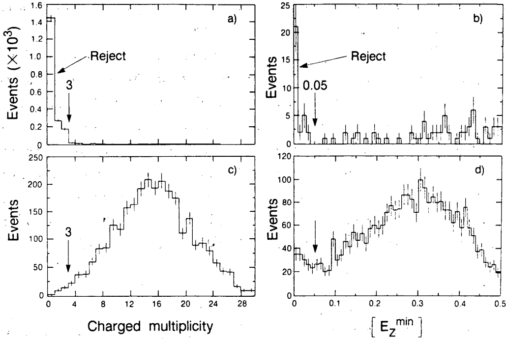
Fig. 13. Charged multiplicity and E_Z^{\min} (see text) distributions for data (a,b), and Monte Carlo (c,d), respectively.
