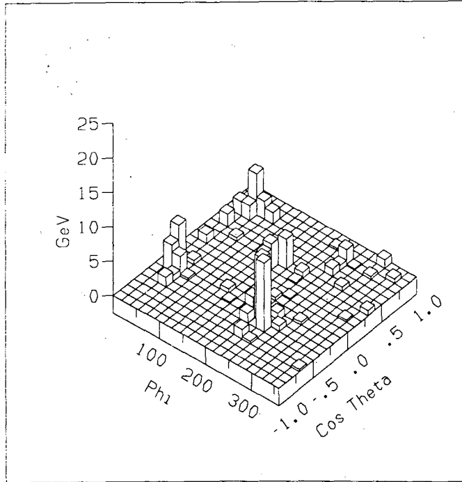
Fig. 22. Leggo plot of a high multiplicity event.
