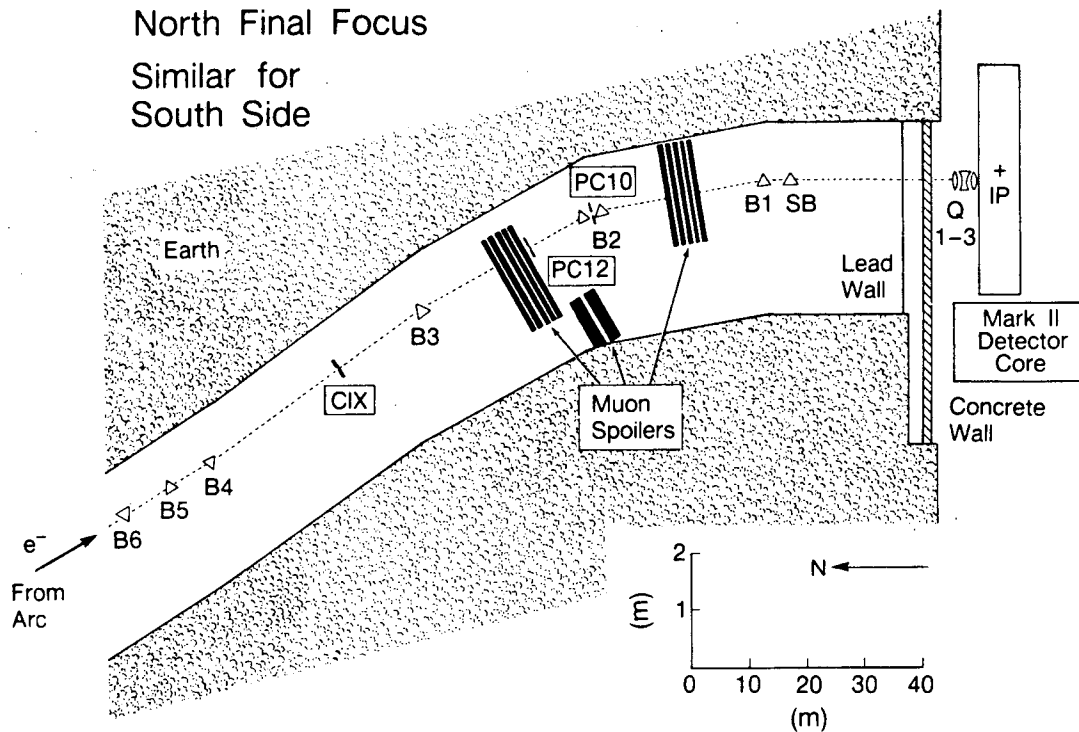
Fig. 2. Collimators and toroids upstream of the IP to reduce background.
