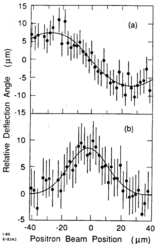
Fig. 4. Measured deflection of the e^+ beam as it is swept in X across the e^- beam (which is displaced 10 \mu\text{m} in Y with respect to the e^+ bunch). a) X deflection. b) Y deflection.
