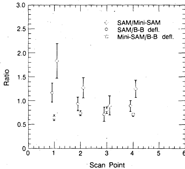
Fig. 11. Luminosity ratios for the various luminosity measuring devices.
