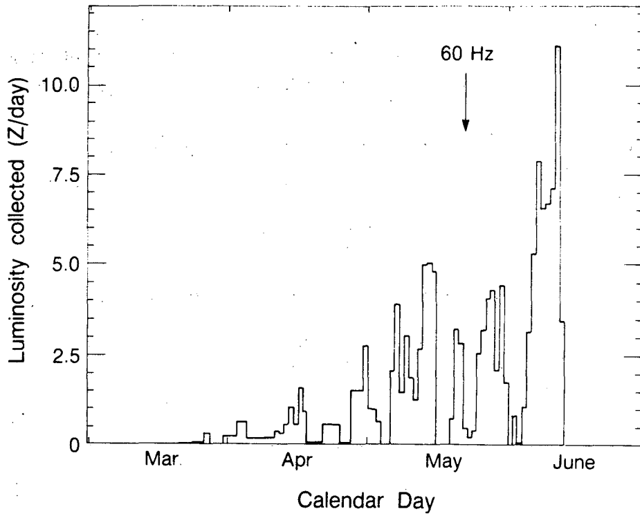
Fig. 6. Daily luminosity, expressed as the number of Z^0 hadronic events which would be produced at the energy set to the mass of the Z^0 .
