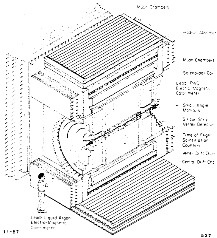
Fig. 8. Pictorial representation of the MARK II at the SLC.
