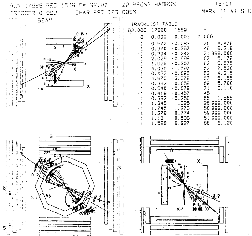
Fig. 14. Transverse view of the central drift chamber and octagonal liquid argon calorimeter for the first hadron observed by the MARK II at the SLC.
