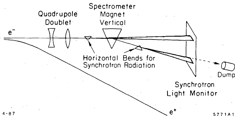
Fig. 12. Extraction line spectrometer used to determine the absolute e^- energy.
