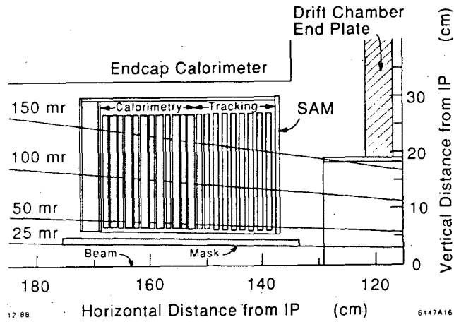
Fig. 10. Schematic drawing of a small angle monitor.
