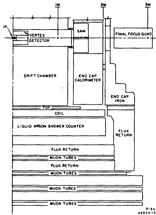
Fig. 9. Schematic representation of the MARK II.
