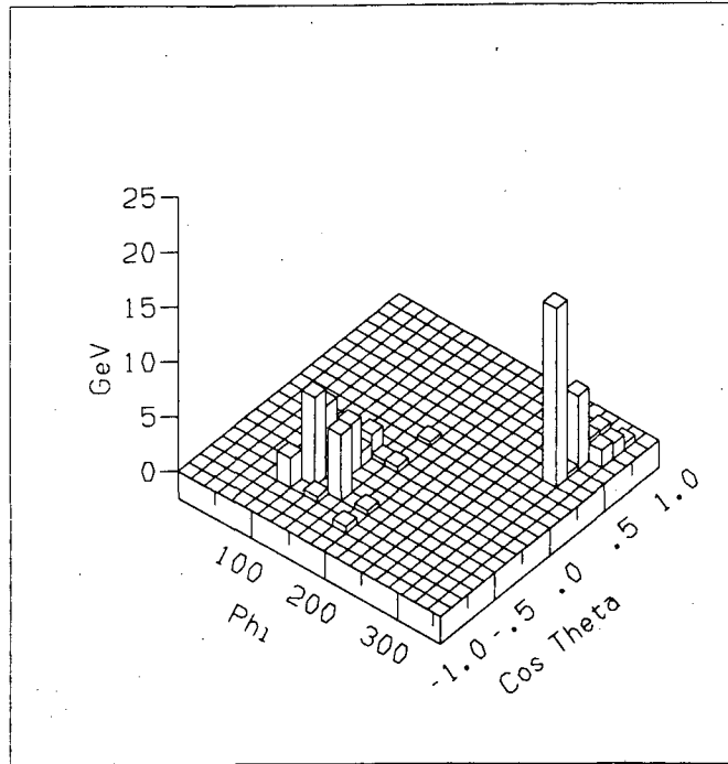
Fig. 16. A lego plot ( \gamma vs. \cos \theta 2-dimensional histogram) for the event shown in fig. 15.
