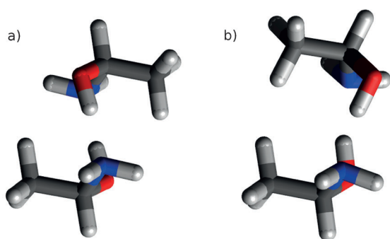
Figure 2. 1-Aminoethanol dimer complexes, stabilized by hydrogen bonds between the amine and hydroxy groups. Complex (a) is formed by molecules of the opposite chirality, while complex (b) contains two molecules of the same chirality. In the latter case, the minimum-energy structure is less compact due to repelling methyl groups.
