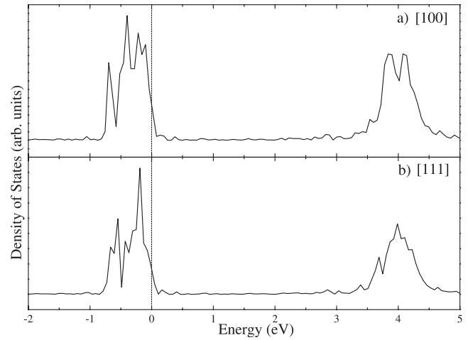
Figure 4. Local density of states (Eu f-states) for atomic displacements along the [100] (a) and [111] (b) directions.
