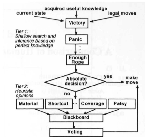
Figure 1: How Hoyle makes decisions.
