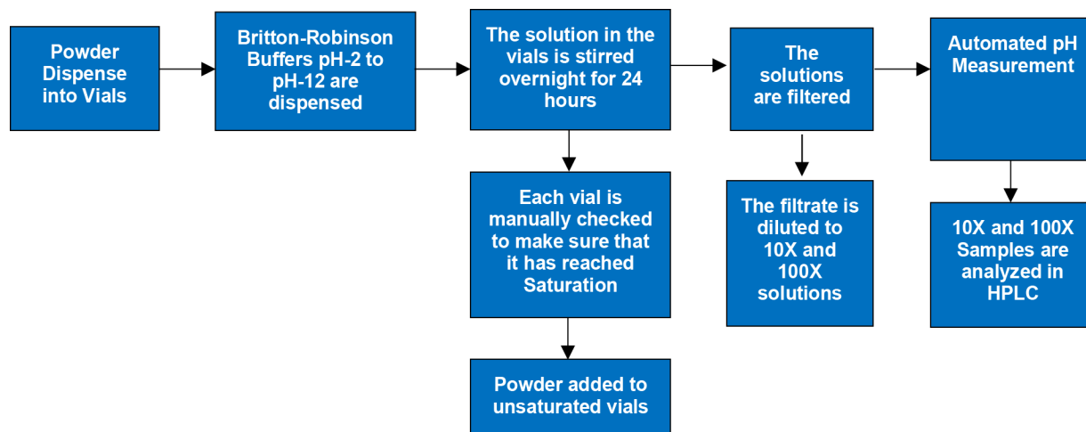
Figure 3. Flow chart of the different steps involved in estimation of experimental pK_a s of compounds.
