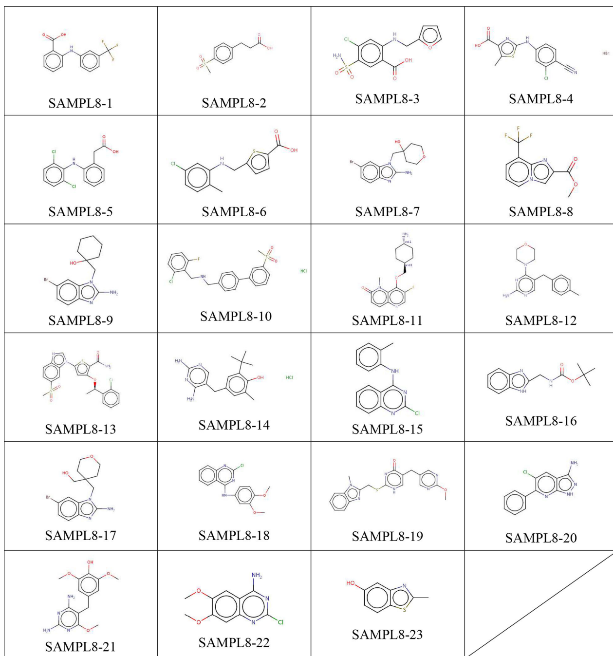
Figure 1. Molecules Used in the SAMP8 pK_a Challenge.
