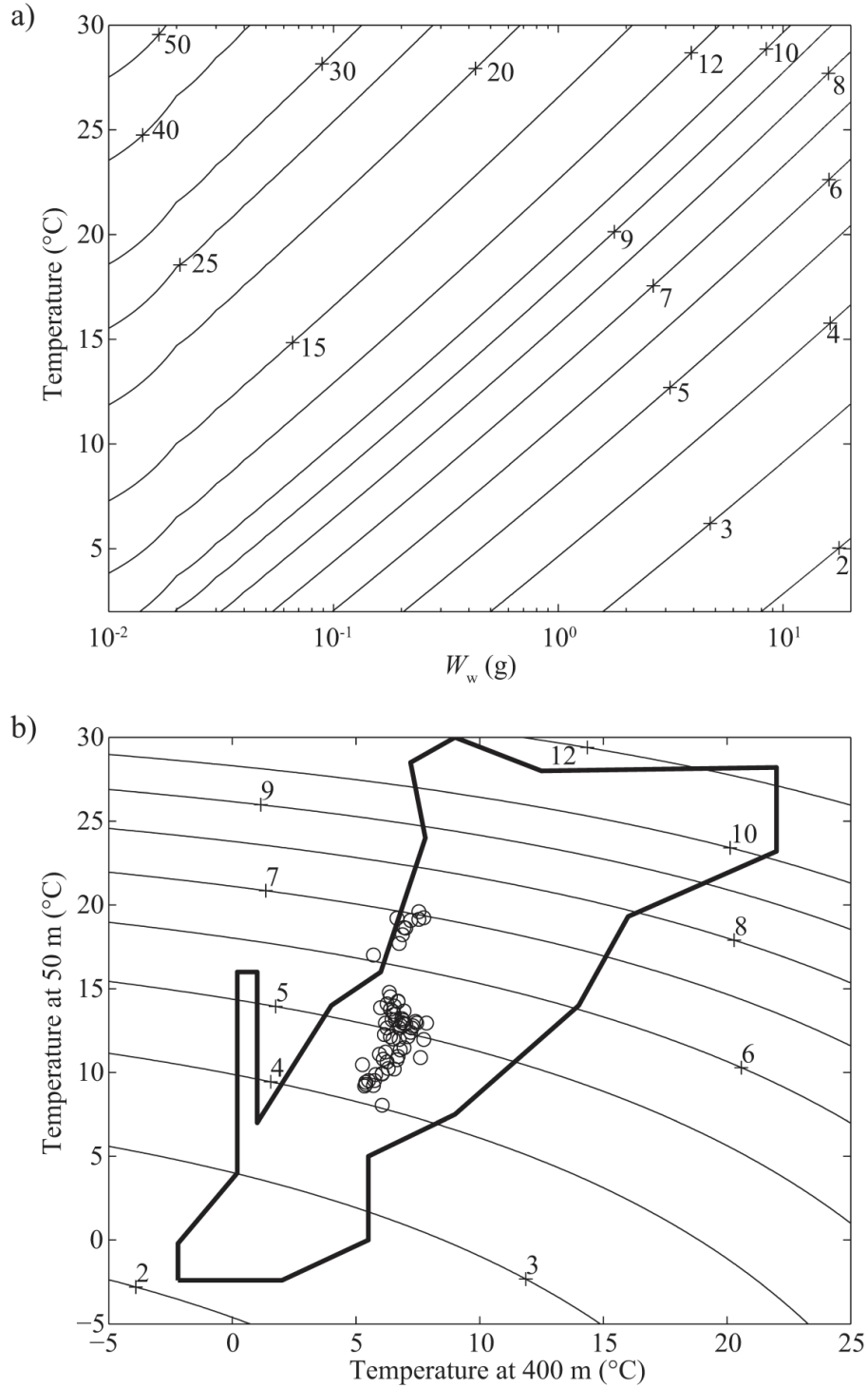
Figure 4.11. Modeled daily ration of fishes; a) effect of wet weight and temperature, b) daily ration of a 2-g vertically-migratory fish (~6 cm L_S ) as a function of temperature at 50 and 400 m depths. The polygon contains the approximate range of these temperatures found in nature (annual average, World Ocean Atlas 2009; Locarnini et al. 2010).
