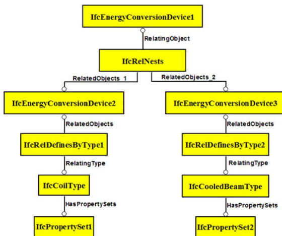
Figure 3 – An example of the concept of containers
