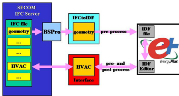
Figure 6 – Diagram of data paths
