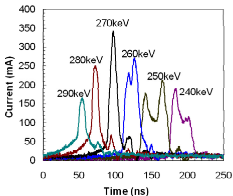
FIG. 5: Compressed beam current pulses using a nominal tilt core voltage waveform as the beam energy is varied.
