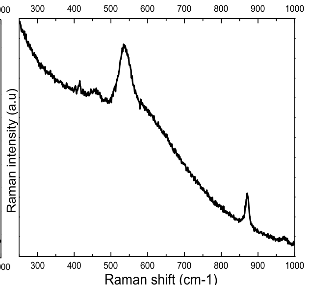
SERS Spectrum for Ni-10Cr-8Fe at E = -0.85V
