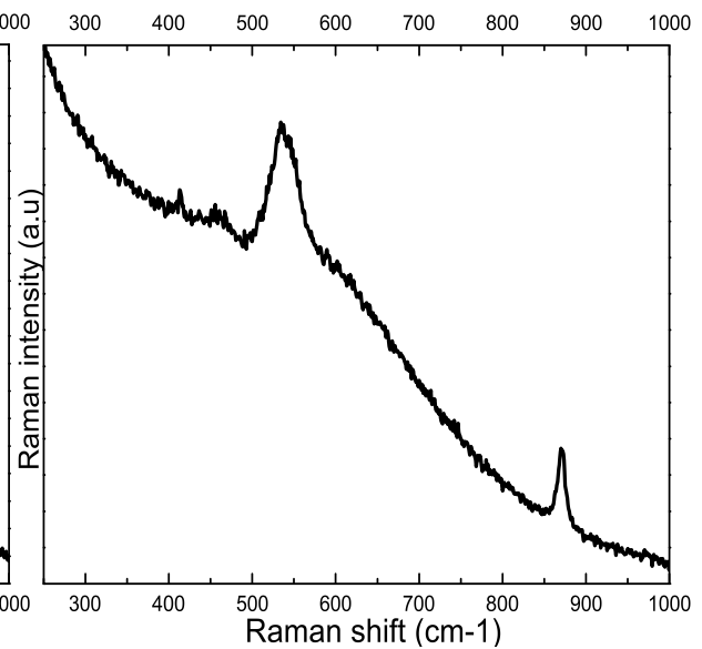
SERS Spectrum for Ni-10Cr-8Fe at E = -0.75V
