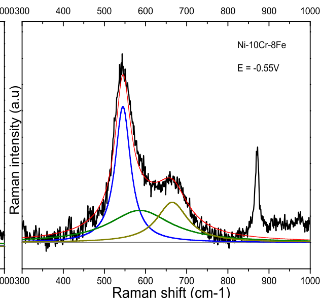
SERS Result for Ni-10Cr-8Fe at E = -0.55V
