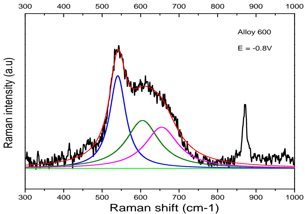
Figure 4-3b. SERS Result for Alloy 600 at E = -0.8V (After Background Subtraction and Peak Fitting)
