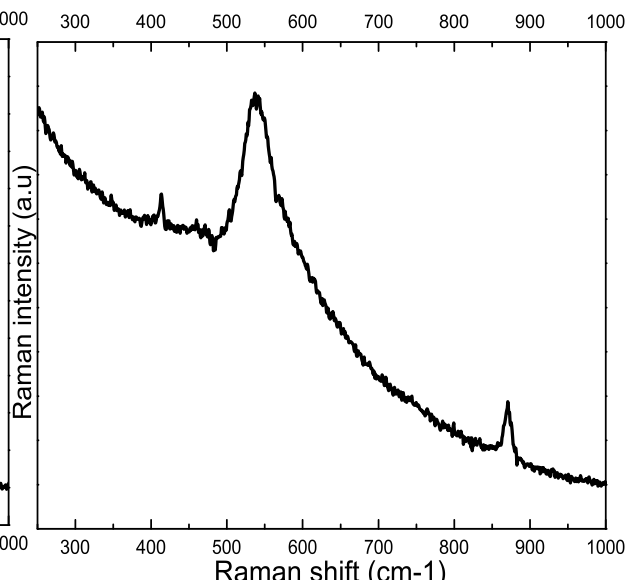
SERS Spectrum for Alloy 690 At E = -0.85V and pH=7.2
