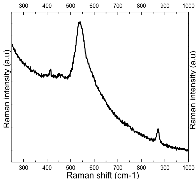
SERS Spectrum for Alloy 690 At E = -0.9V and pH=7.2
