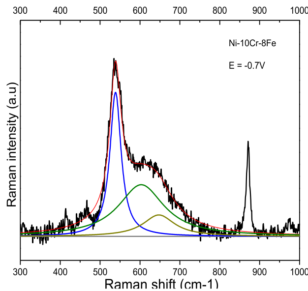
SERS Result for Ni-10Cr-8Fe at E = -0.7V
