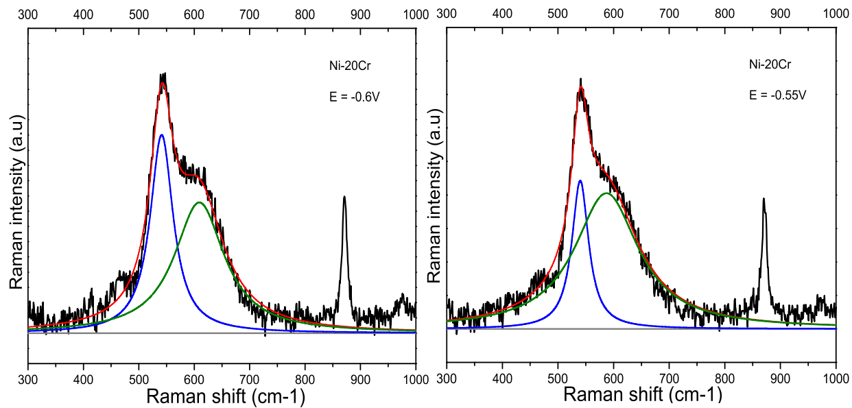
SERS Result for Ni-20Cr at E = -0.55V
