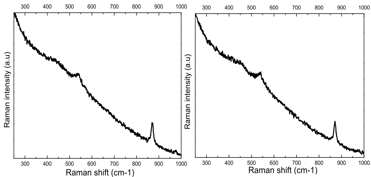
SERS Spectrum for Nickel at E = -0.75V
