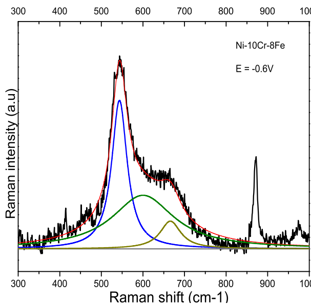
SERS Result for Ni-10Cr-8Fe at E = -0.6V
