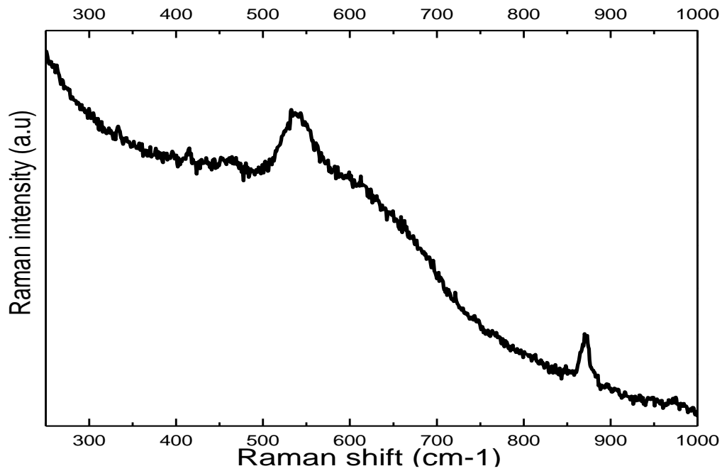
Figure 4-3a. SERS Spectrum measured for Alloy 600 at E = -0.8V
