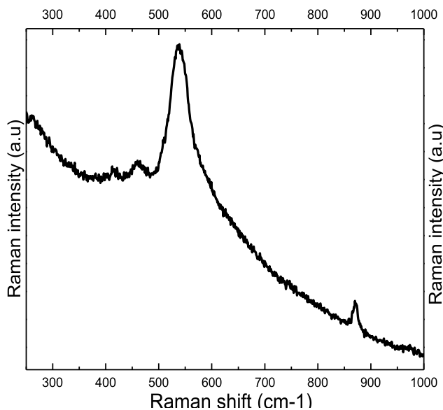
SERS Spectrum for Alloy 690 At E = -0.55V and pH=6.2
