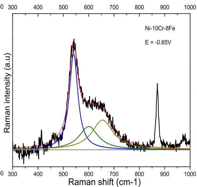
SERS Result for Ni-10Cr-8Fe at E = -0.65V
