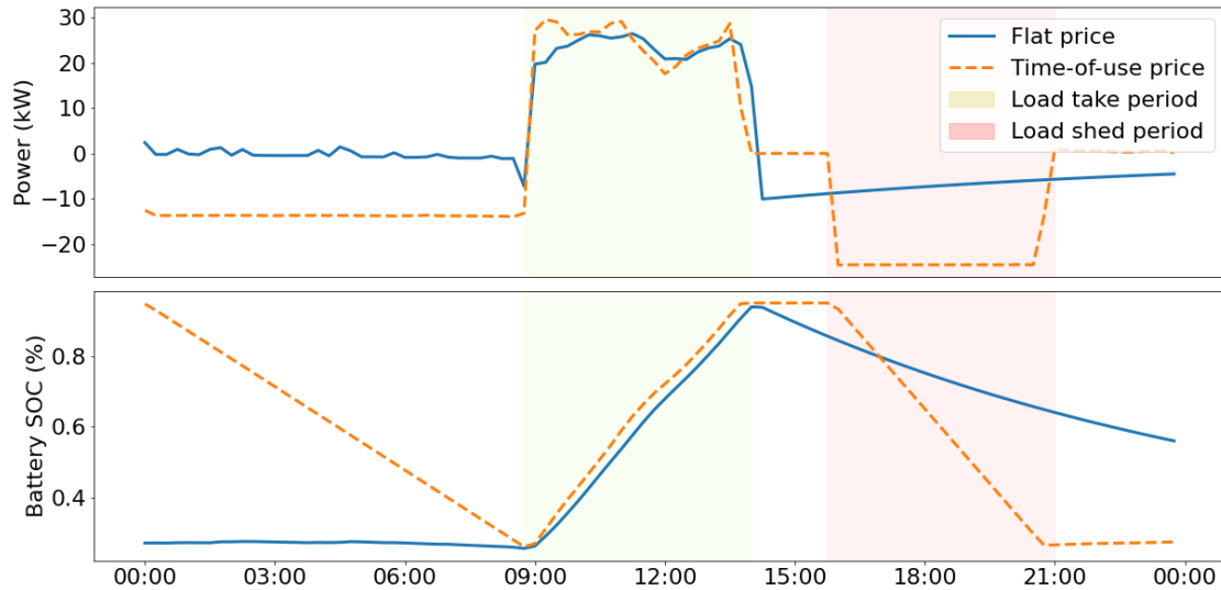
Figure 6: Load shifting battery behavior under a flat price signal and a TOU energy price signal reinforcing the load signal. Battery power (top) and battery SOC (bottom)
