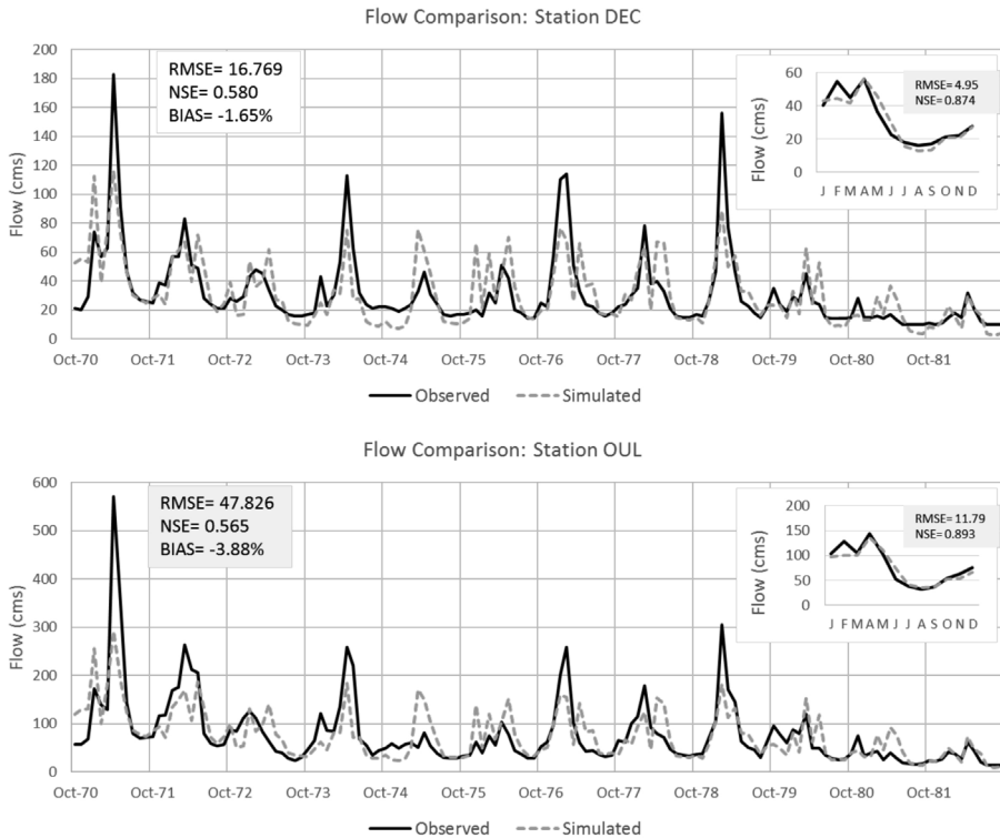
Fig. 8. Hydrologic model calibration results of two gauging stations Dechra el Oued (top) and Oulad Sidi Driss (bottom). The inner figures show observed and simulated monthly cycles.
