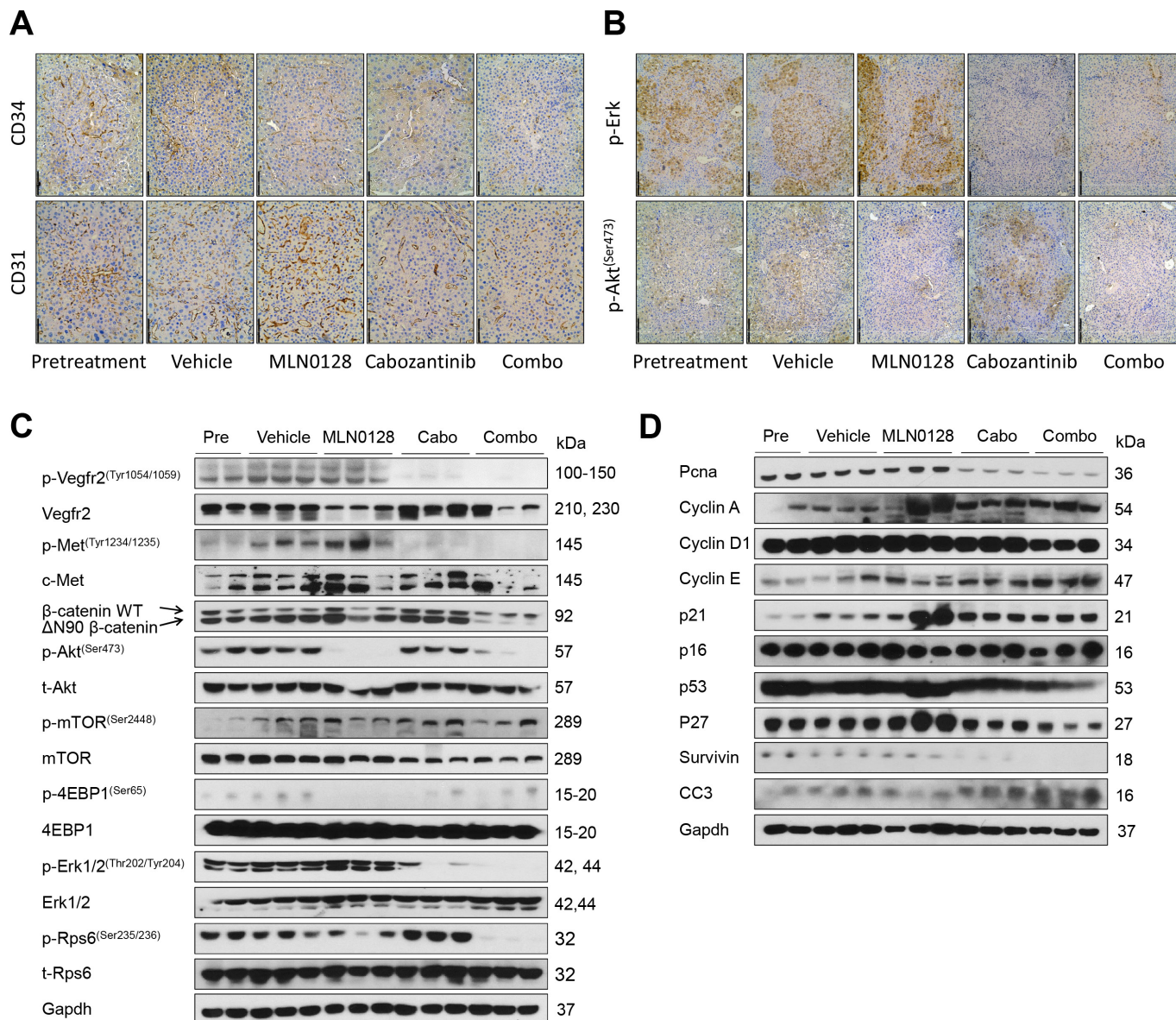
Figure 8 Effect of combined cabozantinib and MLN0128 treatment on tumour microvascular density and putative target proteins in livers from c-Met/β-catenin mice. (A) CD34 (magnification \times 200 ; scale bar=100 \mu\text{m} ) and CD31 (magnification, \times 200 ; scale bar=100 \mu\text{m} ) staining in livers from c-Met/β-catenin mice. (B) p-Akt (Ser473) (magnification \times 100 ; scale bar=200 \mu\text{m} ) and p-Erk (magnification, \times 100 ; scale bar=200 \mu\text{m} ) staining in livers from c-Met/β-catenin mice. Western blot analysis was performed to determine the levels of phosphorylated Vegfr2, phosphorylated c-Met, Akt/ mTOR and MAPK (C), as well as proliferation and apoptosis markers (D) in c-Met/β-catenin mice. Cabo, Cabozantinib; CC3, cleaved caspase 3; combo, combined cabozantinib/MLN0128 treatment.
