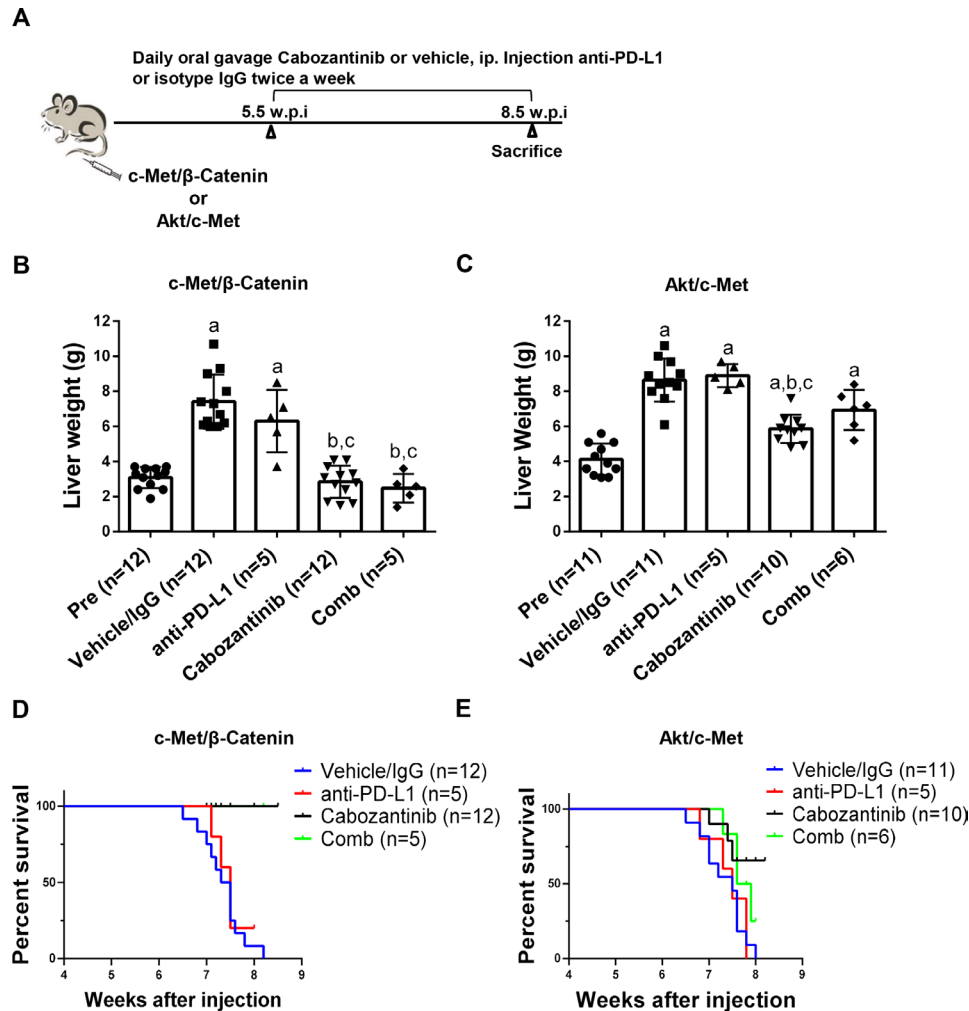
Figure 9 Effect of combined cabozantinib and anti-PD-L1 treatment in c-Met/ \beta -catenin mice and Akt/c-Met mice. (A) Study design. (B) Liver weight of pretreatment-treated, vehicle/isotype IgG-treated, cabozantinib-treated, PD-L1-treated and cabozantinib/anti-PD-L1-treated c-Met/ \beta -catenin mice. (C) Liver weight of pretreatment-treated, vehicle/isotype IgG-treated, cabozantinib-treated, PD-L1-treated and cabozantinib/anti-PD-L1-treated Akt/c-Met mice. (D-E) Survival curve of c-Met/ \beta -Catenin and Akt/c-Met mice treated with vehicle/isotype IgG, Cabozantinib, PD-L1 and Cabozantinib/anti-PD-L1. Tukey–Kramer test: at least p < 0.05 . a, versus pretreatment; b, versus vehicle; c, versus anti-PD-L1. Cabo, cabozantinib; Comb, combined cabozantinib and anti-PD-L1 treatment; Pre, pretreatment.
