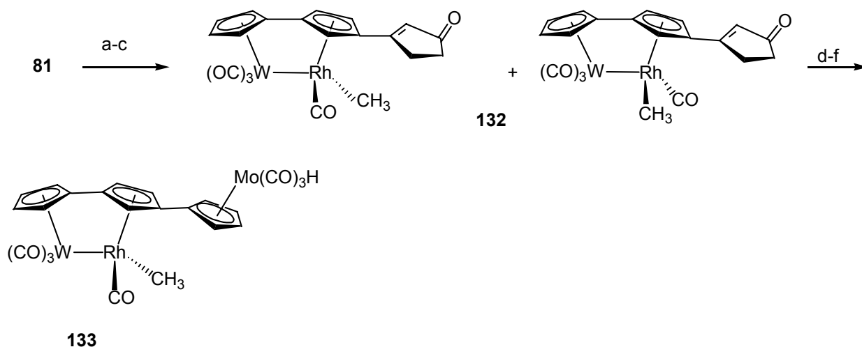
Scheme 29 a) NaH; b) 3-chlorocyclopentenone; c) NaH, THF, [Rh(CO) 2 Cl] 2 , -20 °C to reflux, column chromatography; d) i BuAlH; e) 4-MeC 6 H 4 SO 3 H; f) Mo(NCt) 3 (CO) 3 .
