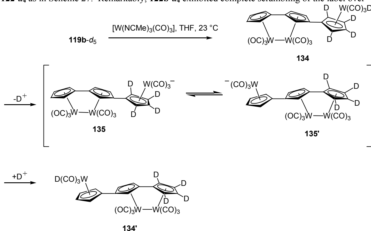
Scheme 30
