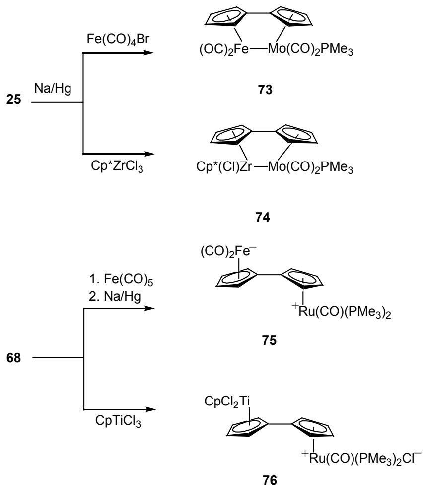
Scheme 18
