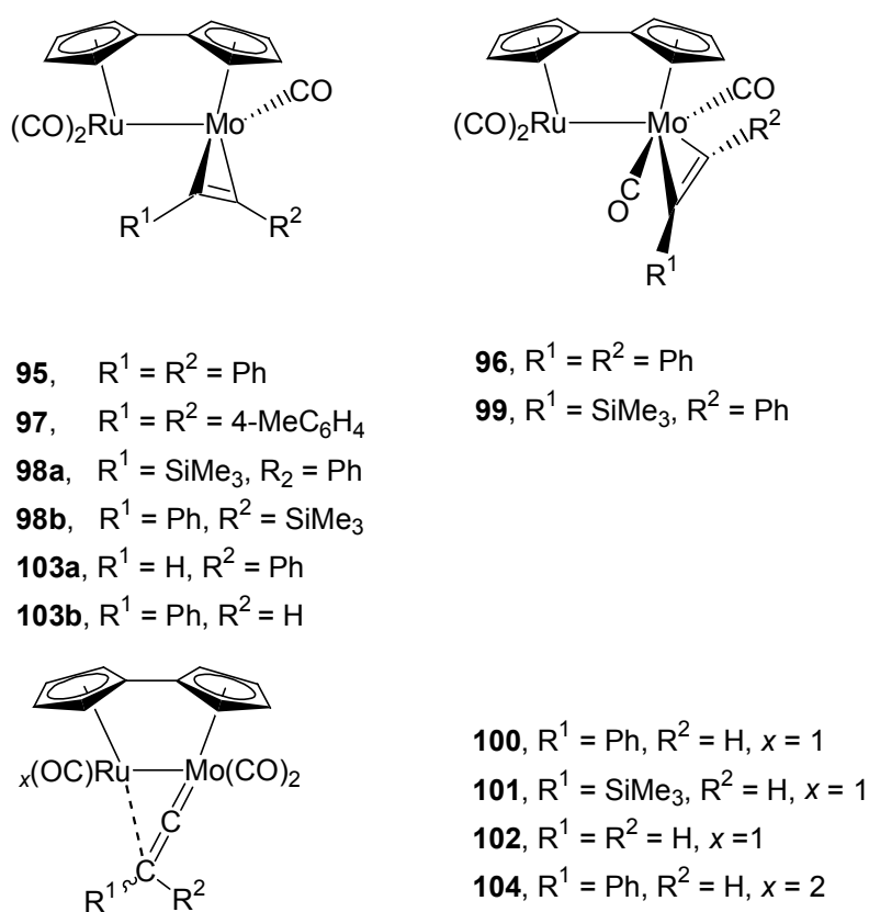
Scheme 21
