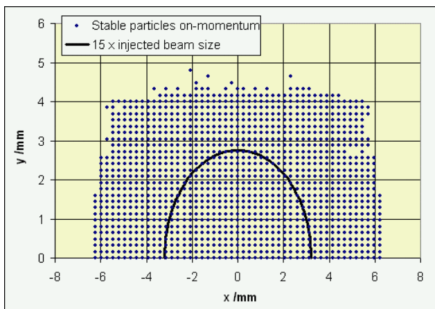
Figure 4: Dynamic aperture for on-momentum particles.
