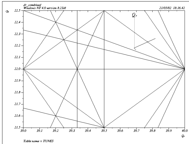
Figure 3: Variation in tunes with momentum deviations up to \pm 2\% .
