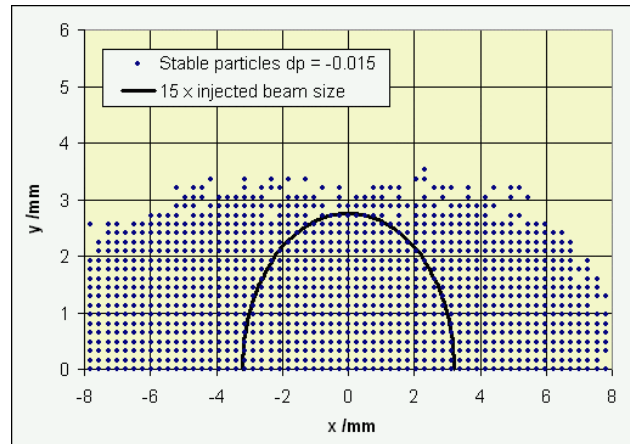
Figure 5: Dynamic aperture for particles with -1.5\% momentum deviation.
