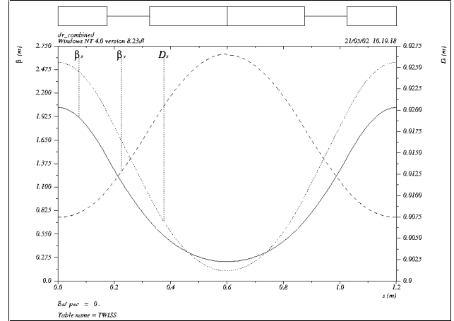
Figure 1: Lattice functions in a single arc cell.
