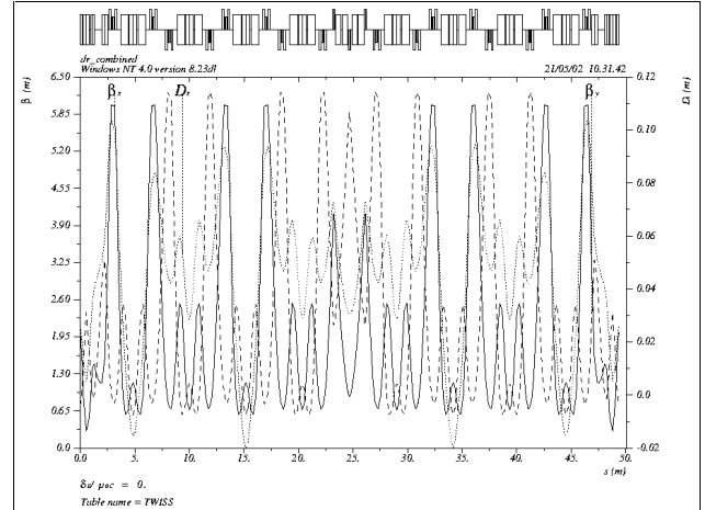
Figure 2: Lattice functions in the chromatic correction section.
