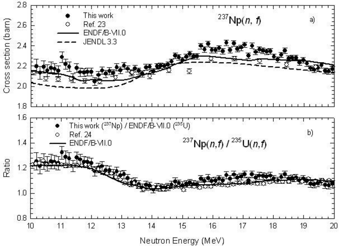
Fig. 6. a) Cross sections for the ^{237}\text{Np}(n, f) reaction and b) Ratio for the ^{237}\text{Np}(n, f) to ^{235}\text{U}(n, f) cross sections of this work along with measured and evaluated data. The ratio for this work in b) was generated using the ^{235}\text{U}(n, f) data from ENDF/B-VII.0. Error bars show only the statistical uncertainty. Note the zero-suppressed horizontal and ordinate axis.
