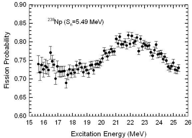
Fig. 4. Measured fission probabilities of the ^{238}\text{Np}^* produced from the ^{238}\text{U}(^3\text{He},f) reaction. Error bars show the statistical uncertainty only. Threshold of ^{238}\text{Np}^* 3 rd chance fission is 18.2 MeV excitation energy.
