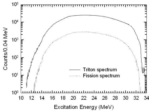
Fig. 3. Integrated singles triton spectrum and background corrected fission spectrum of the particle telescope and fission detector. The reported 10 to 20 MeV equivalent neutron energy range of this work corresponds to \sim 15.5 to \sim 25.5 MeV ^{238}\text{Np}^* excitation energy.
