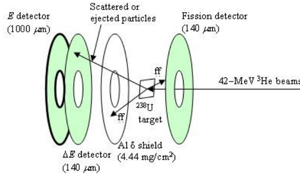
Fig. 1. Experimental setup of ^{238}\text{U} target, silicon telescope ( \Delta E+E ), Al shield, and fission detector. The target was placed 15 mm upstream from the telescope and the fission detector was 10 mm upstream from the target. Arbitrary directions for the scattered/ejected particle and fission fragment (ff) along with the incoming beam on the ^{238}\text{U} target are shown.
