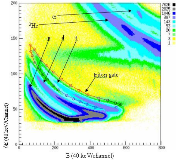
Fig. 2. \Delta E vs. E plot for a single ring at 49^\circ with respect to the beam axis shows different ejected particles from the interaction of 42-MeV ^3\text{He} beams with the ^{238}\text{U} target. Protons ( p ), deuterons ( d ), and tritons ( t ) are located in the lower left side in the plot and part of the ^3\text{He} and \alpha particles are visible in the upper right corner in the plot. A typical triton gate is shown. The horizontal band at \Delta E \sim channel 125 represents ^3\text{He} particles of incomplete energy deposition including random particles in coincidence with the elastic peak. The channel cut below \Delta E \sim channel 30 was due to sort routine parameter setup.
