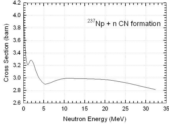
Fig. 5. Calculated ^{237}\text{U} + n compound nucleus formation cross section
