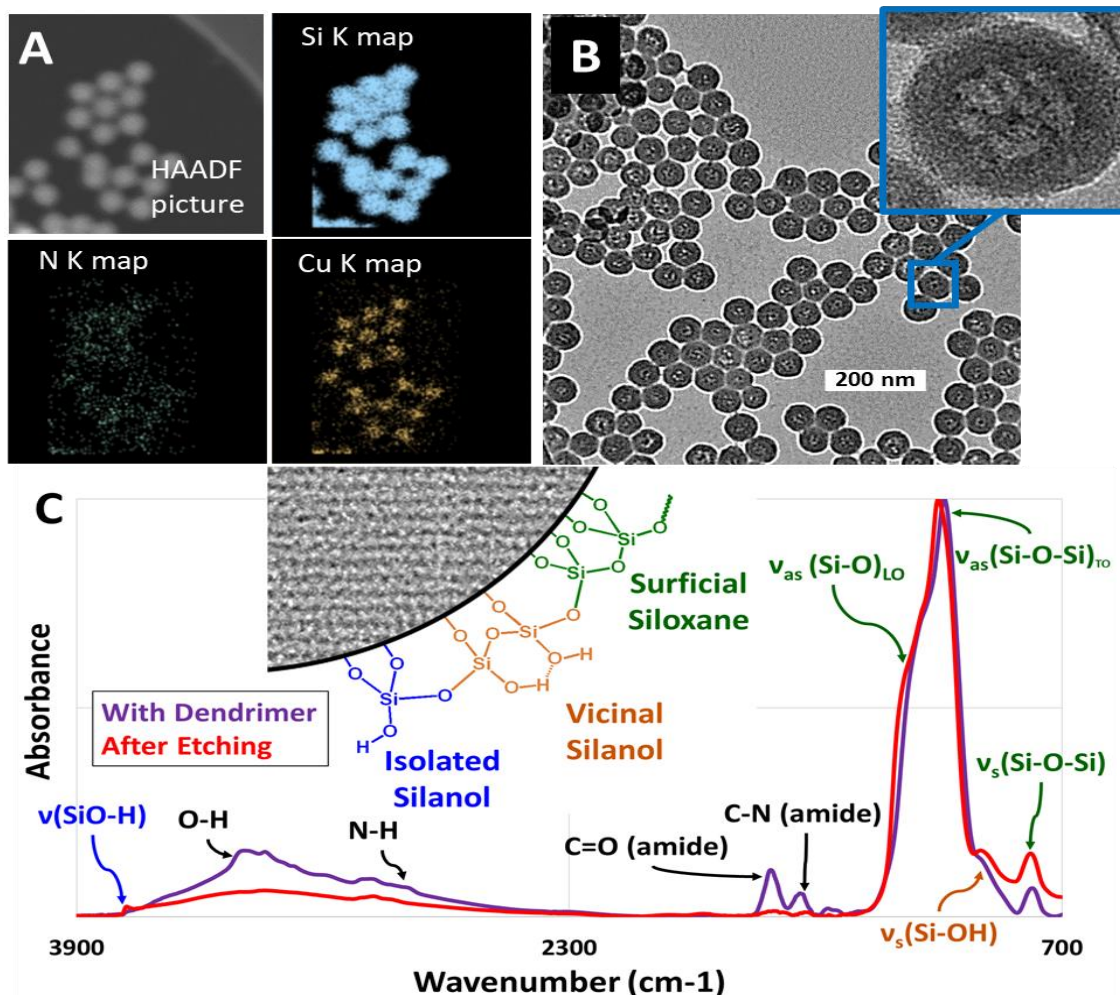
Figure 2: Figure shows (A) STEM/EDS phase maps for Cu encapsulated G 4 OH in microporous silica nanoparticles (NPs), (B) TEM picture of silica inorganic micelles after removal of the metal and dendrimer with enlarged inset of single NP, and (C) FTIR spectra of as-synthesized silica NPs before (purple) and after (red) the removal of Cu 2+ and G 4 OH. Inset defines functional group variations at the silica surface.
