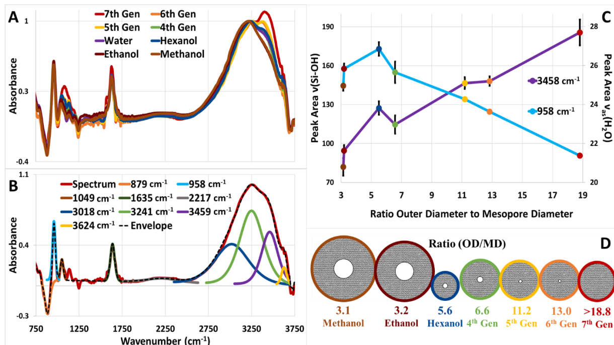
Figure 6: Figure shows (A) representative FTIR spectral series of the hydration of all synthesized nanoparticle species, and (B) representative FTIR spectrum of the vibrational energies of water as individually fit. (C) Plot of the vibrational stretching regions of water, and the hydration of the surface silica, as they change as a function of the ratio of outer to inner nanoparticle diameter. (D) A visual representation of the ratio of the outer diameter to the internal mesopore diameter.
