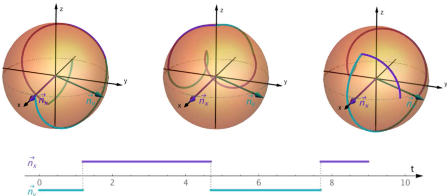
Fig. 6 Time-optimal control solution to obtain a \pi rotation about the \mathbf{n}_z axis for \alpha = \pi/3 and \kappa = 3/4 . The time-optimal solution is represented in a similar way to Fig. 5. It can be applied to any initial state \mathbf{r}(0) : left , \mathbf{r}(0) = \mathbf{n}_x ; center , \mathbf{r}(0) = \mathbf{n}_z (so no net rotation is obtained); right , \mathbf{r}(0) = (\mathbf{n}_x + \mathbf{n}_y)/\sqrt{2}
