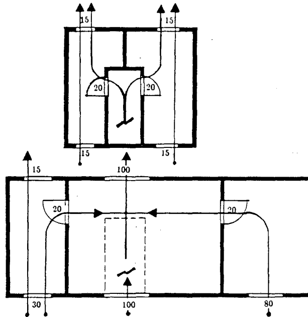
Fig. 7: Assumed flow paths - 1. iteration step
