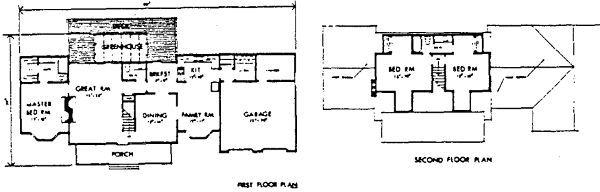
Fig. 6: Two-story single family building
