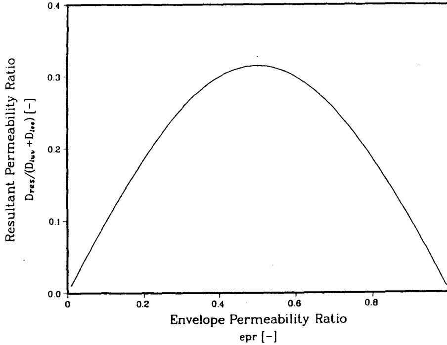
Fig. 3: Resultant permeability ratio versus envelope permeability ratio
