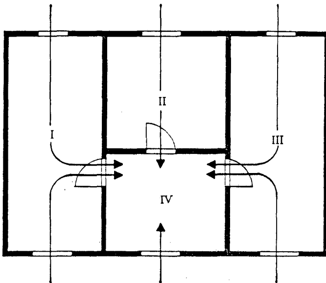
Fig. 5.6: Flowpaths below n_z due to stackeffect
