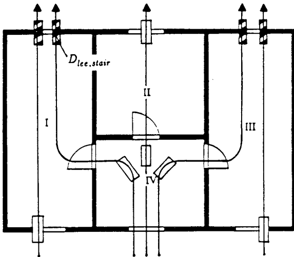
Fig. 5.4: Step #6 - Splitting D_{lee} to find D_{lee,stair}
