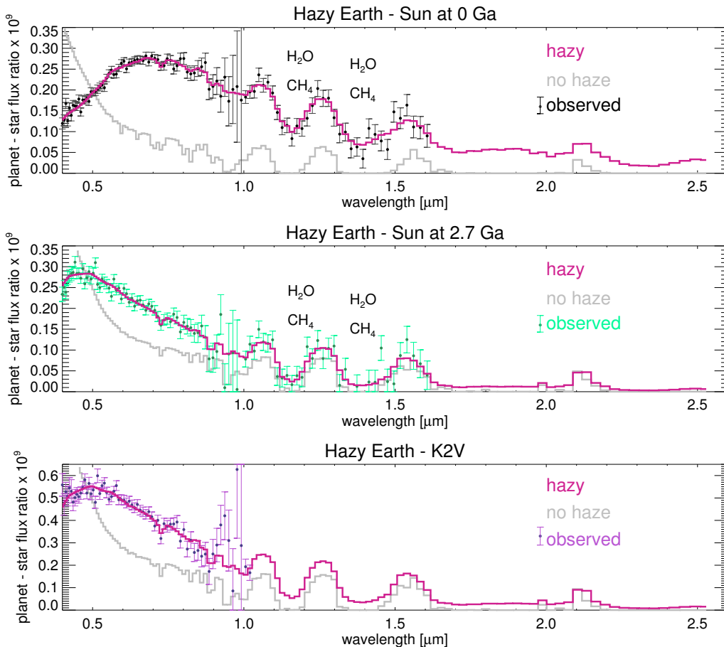
Figure 9. These are simulated reflectance spectra as seen by a 10-m LUVIOR-type telescope over 200 hours of integration time in each spectral band for planets at 10 pc. The colored lines show the hazy spectra without noise added, and the gray spectra are the corresponding haze-free planets for comparison. Points with error bars simulate the hazy spectrum seen by the telescope with realistic noise sources.
