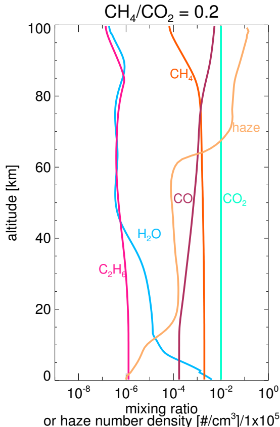
Figure 3. The gas profiles for the nominal atmosphere investigated by this study for \text{CH}_4/\text{CO}_2 = 0.2 and p\text{CO}_2 = 0.01 bar for a planet orbiting the Archean sun (2.7 Ga).
