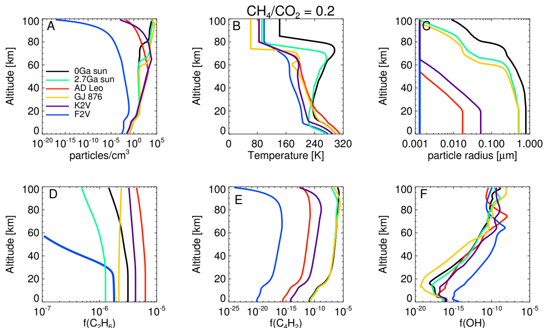
Figure 4. Displayed here are: A) the number density of haze particles, B) the temperatures of the \text{CH}_4/\text{CO}_2 = 0.2 atmospheres, C) radii of haze particles, D) the \text{C}_2\text{H}_6 mixing ratios, E) the mixing ratio of \text{C}_4\text{H}_2 particles, which is the primary vector that condenses directly out to form aerosols in our chemical scheme, and F) the mixing ratio of OH radicals, to illustrate the buildup of such oxygen species in the atmosphere of the F star.
