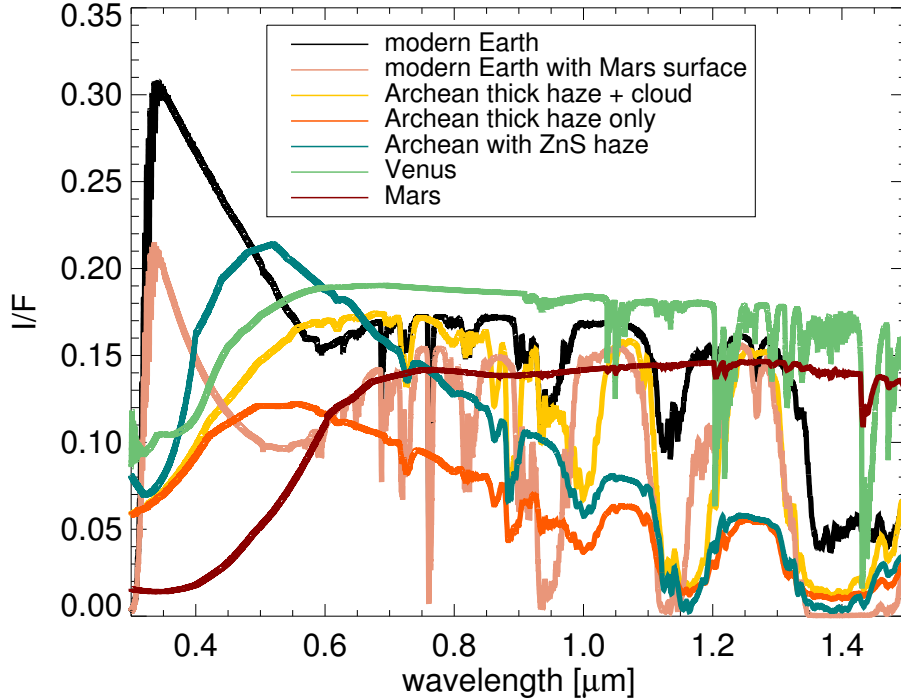
Figure 10. This shows a comparison of several types of spectra with broad short wavelength absorption features to compare haze’s short wavelength absorption feature to similar features produced by different types of absorbers. These spectra have been scaled in the y-dimension to plot together on the same axis.
