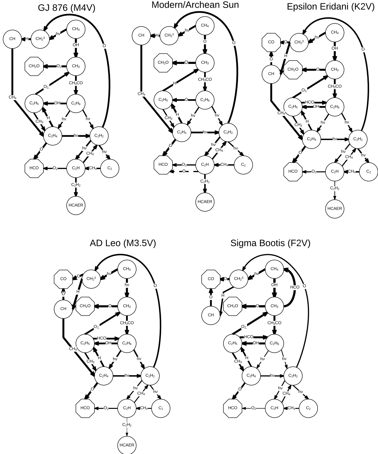
Figure 5. The fastest reaction network towards haze formation (HCAER) and the fastest hydrocarbon sinks for each planet. The Archean and modern sun reaction networks are the same except for the reaction forming \text{HCO} from \text{C}_2\text{H} : the dominant reaction involves \text{O}_2 for the modern sun (solid arrow) and \text{O} for the Archean sun (dashed arrow). The F2V star, on the other hand, has a complex network in which hydrocarbons efficiently react with oxygen species, and haze is not formed. Thicker arrows indicate faster reaction rates.
