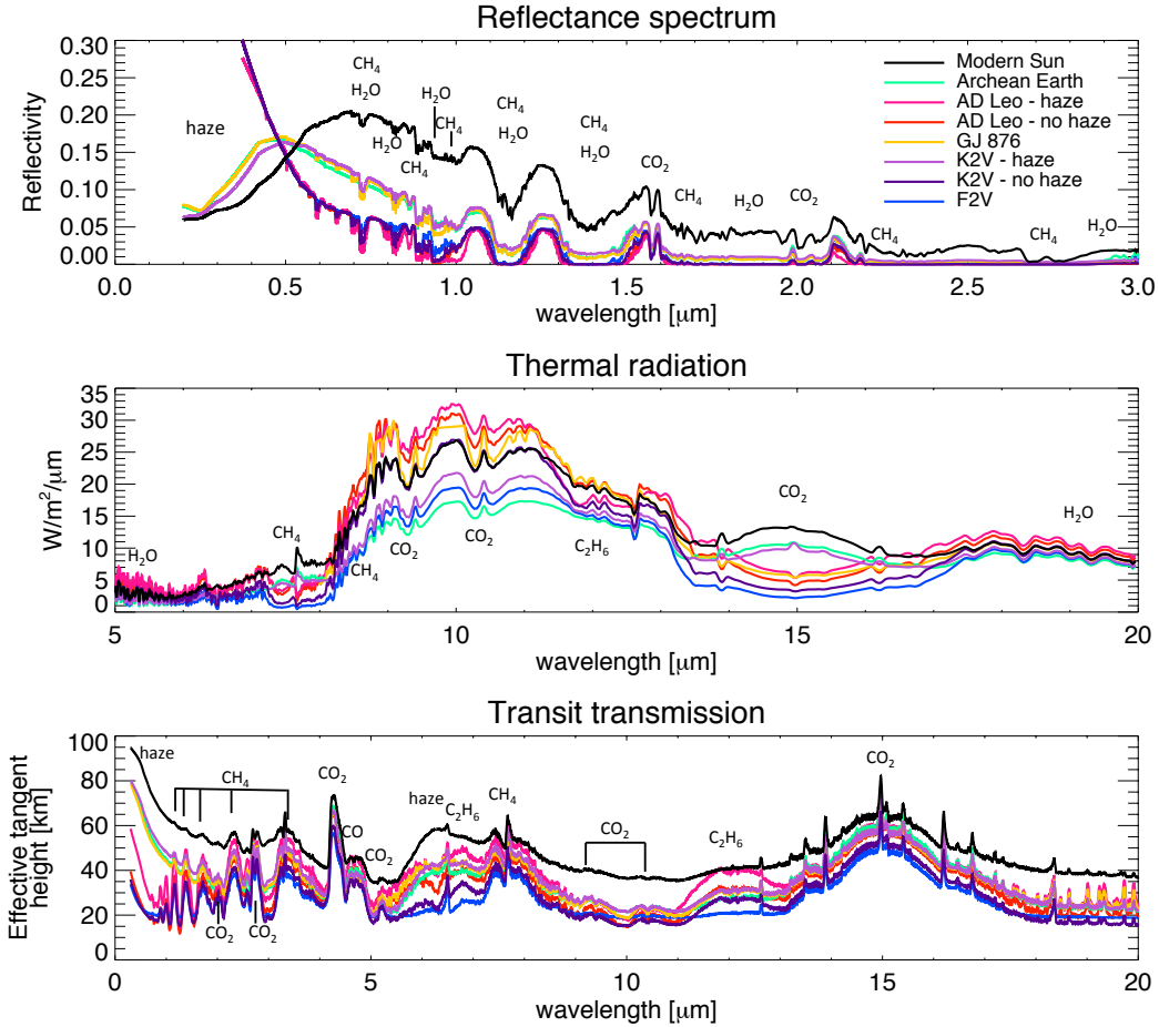
Figure 6. Reflectance spectra (top panel), thermal radiation (middle panel) and transit transmission spectra (bottom panel) for the Archean Earth-type planets around varied spectral types. The transit transmission spectra show the effective tangent height, which is the minimum altitude the atmosphere is transparent to as a function of wavelength for light traveling tangent to the planet surface. All spectra shown are for \text{CH}_4/\text{CO}_2 = 0.2 except spectrum labeled “K2V - haze”, which has \text{CH}_4/\text{CO}_2 = 0.3 , and the “AD Leo - haze” spectrum, which has \text{CH}_4/\text{CO}_2 = 0.9 .
