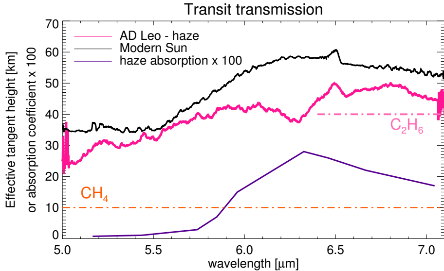
Figure 7. A zoom in on the region around 6 \mu\text{m} showing the transit transmission spectra of the modern Sun planet, which has the most optically thick haze of all the planets studied here, and the “AD Leo - haze” spectrum, which has a very thin haze but the largest amount of \text{C}_2\text{H}_6 . The purple solid line shows the haze extinction coefficient ( k ) scaled by a factor of 100 to plot on the same y-axis, and the peak in this curve corresponds to the peak in the “modern Sun” spectrum. Dot-dashed lines show the wavelength ranges where \text{CH}_4 and \text{C}_2\text{H}_6 absorb. Absorption from haze occurs near 6.3 \mu\text{m} in the “modern Sun” spectrum, and absorption from \text{C}_2\text{H}_6 prominently occurs between 6.5 and 7 \mu\text{m} for the “AD Leo - haze” spectrum.
