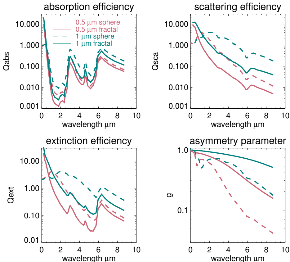
Figure 1. The absorption efficiency ( Q_{abs} ), scattering efficiency ( Q_{sca} ), extinction efficiency ( Q_{ext} = Q_{abs} + Q_{sca} ), and the asymmetry parameter ( g ) as a function of wavelength for 0.5 \mu\text{m} (pink) and 1 \mu\text{m} (teal) fractal (solid lines) versus spherical (dashed lines) particles. g is a measure of the degree of particle forward scattering; a value of 1 would indicate perfect forward-scattering, while 0 would indicate perfectly isotropic scattering. Fractal particles produce more extinction at short wavelengths than equal mass spherical particles, and they also tend to be more forward scattering. This diminishes their ability to cool the planet by allowing longer wavelengths to be transmitted to the surface. We assume optical constants from Khare et al. (1984).
