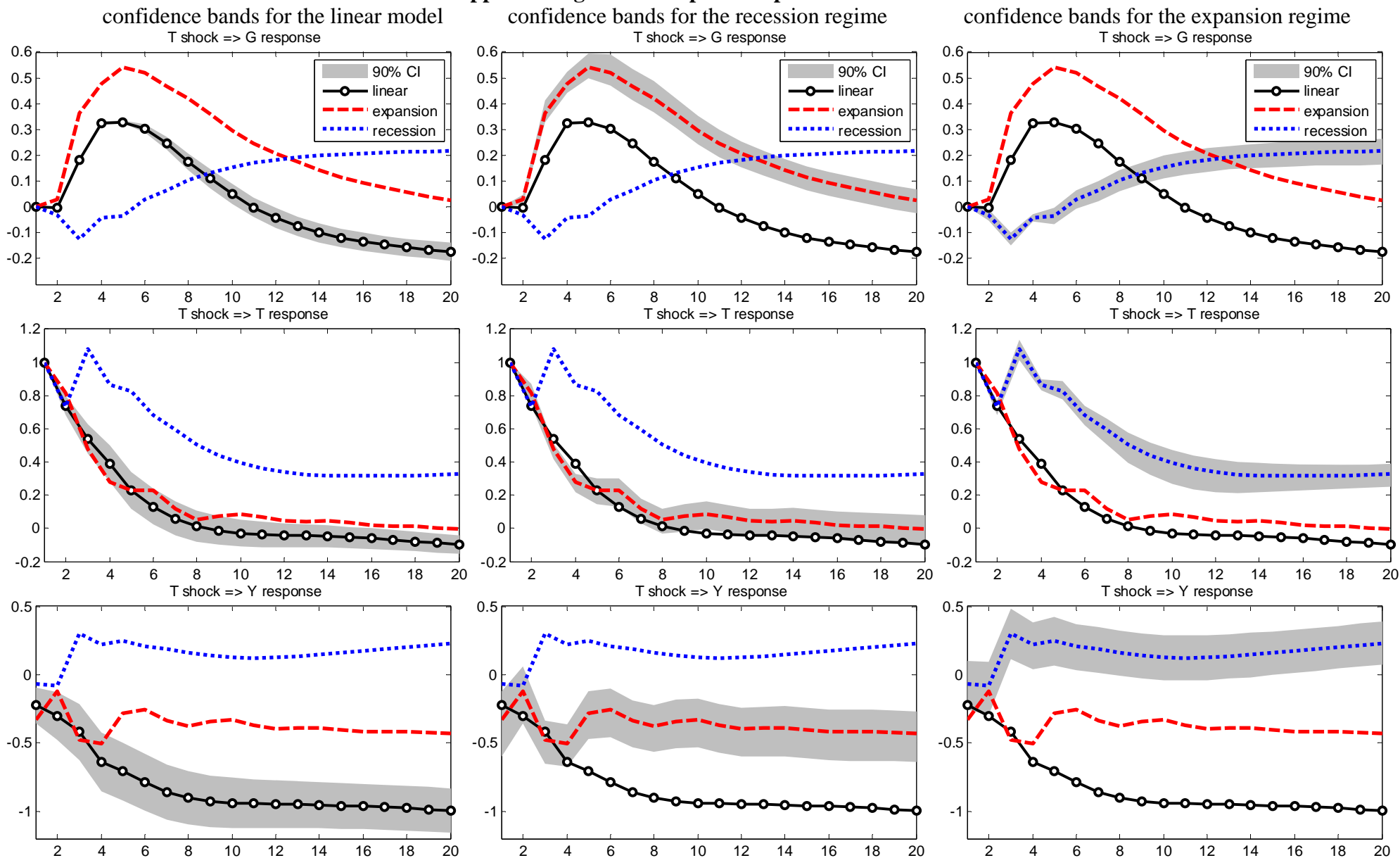
Appendix Figure A1. Impulse responses to tax shocks
