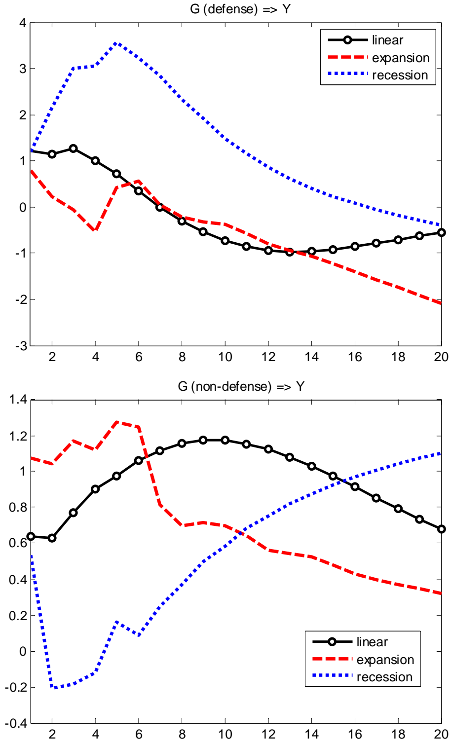
Figure 4. Defense and nondefense government spending
