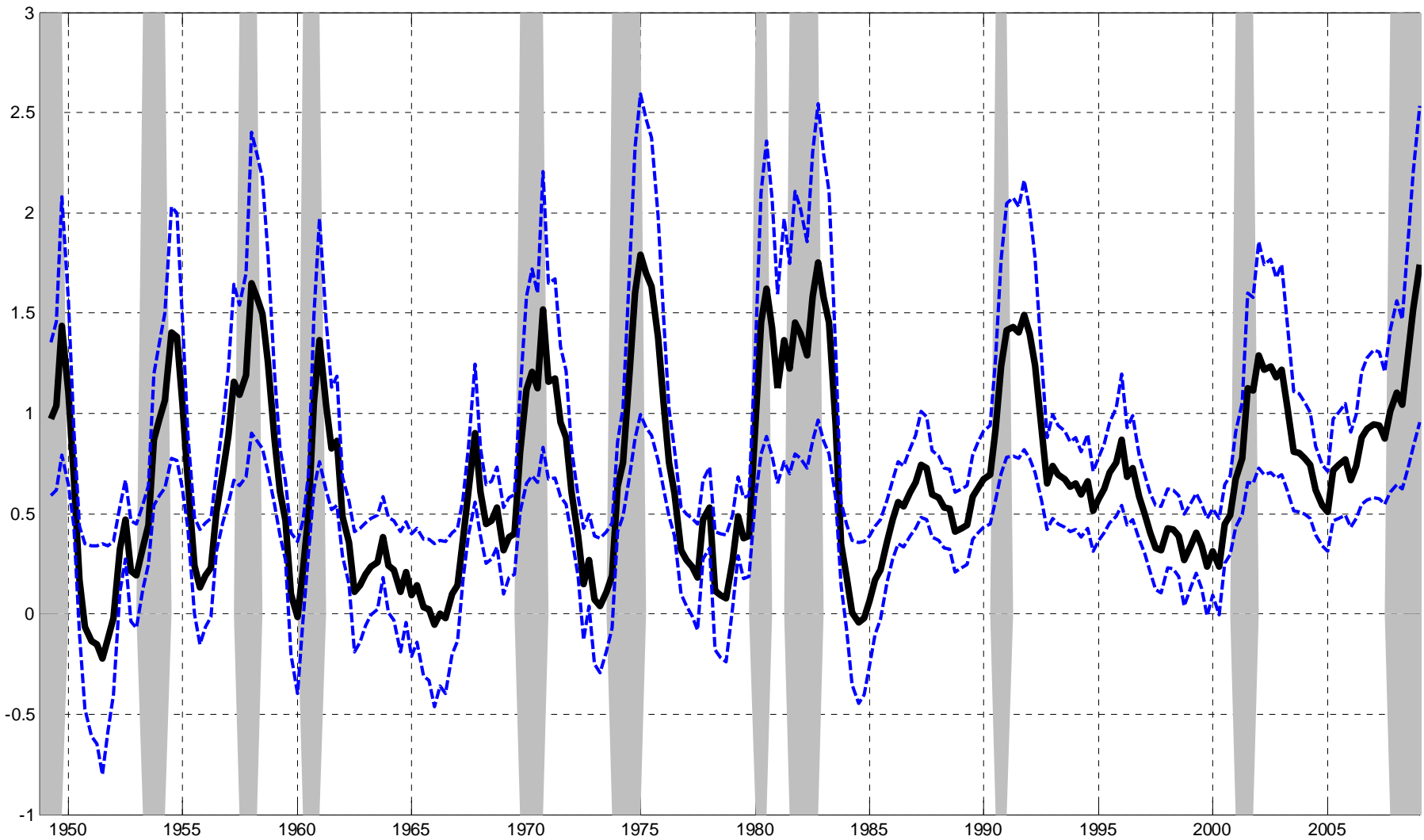
Figure 3. Historical multiplier for total government spending
