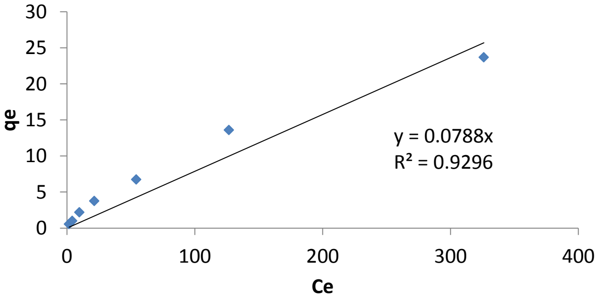
Norit 1240 Linear Isotherm Fit at 30°C
