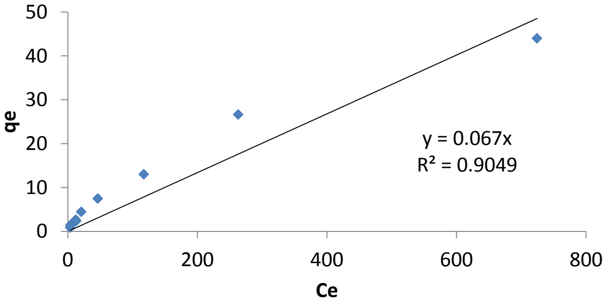
Norit 1240 Linear Isotherm Fit at 20°C
