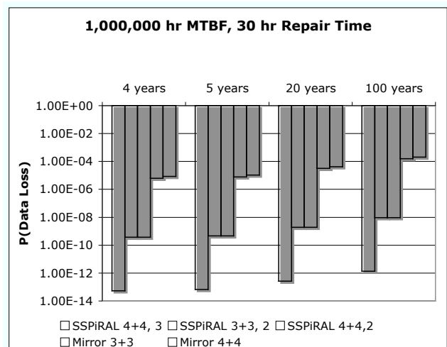
Figure 13. Data loss probability for SSPiRAL and Mirrored layouts with equivalent space efficiency and a 30 hour repair time.
