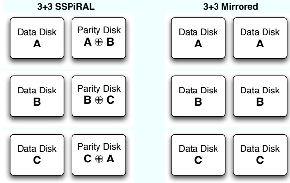
Figure 1. 3+3 SSPiRAL Layout vs. 3+3 Mirrored Disk.
