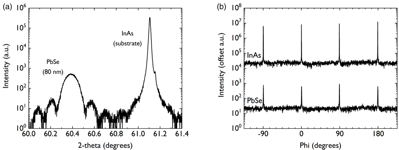
FIG. 7. Crystallinity of PbSe films on InAs: (a) 2\theta - \omega coupled scan of the (004) peak showing a high-quality interface with distinct thickness fringes. (b) A 360^\circ \phi -scan of the \{224\} peaks in PbSe and InAs, showing that the nominal epitaxial registration between the film and substrate is (001) cube-on-cube.
