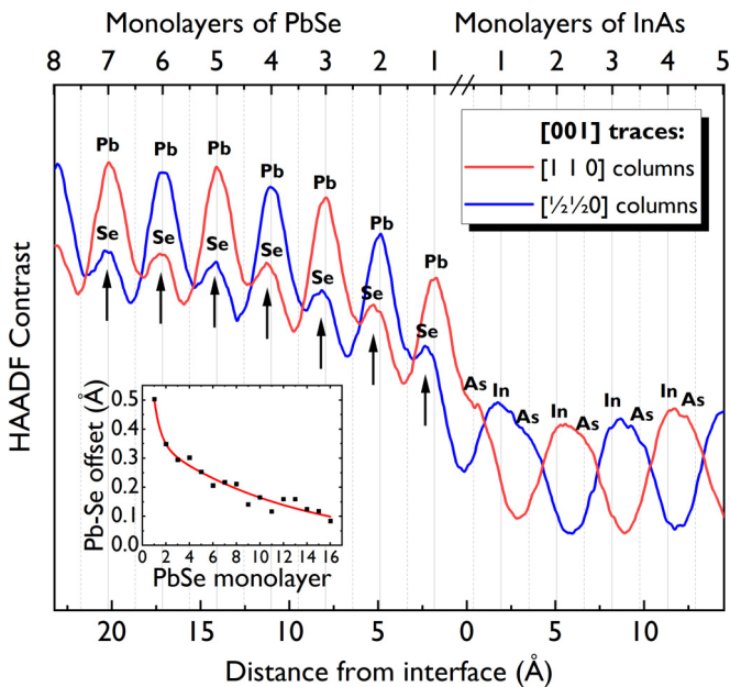
FIG. 4. [001] contrast traces (averaged without fitting) across the HADDF STEM micrograph from Fig. 3 (left). The InAs barbellis can be seen on the right, and the alternating Pb/Se species on the left. At the interface, the final InAs layers appear slightly stretched, and the first few monolayers of the selenium sublattice are warped away from the interface. The vertical grid lines are at a regular interval.
