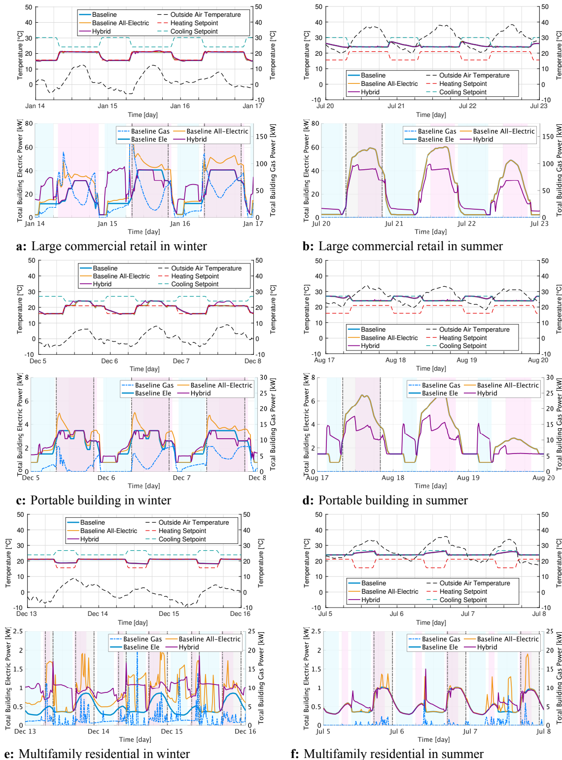
Figure 3: Three systems in winter and summer where grey vertical lines enclose peak tariff periods, blue shaded regions correspond to TES charge windows, and pink shaded regions correspond to TES discharge windows
