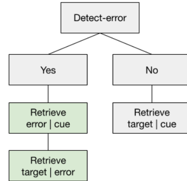
Figure 2: Using an additional production rule to model mediator error learning.
