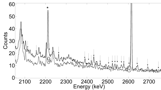
FIG. 3: NRF spectrum of the ^{240}\text{Pu} target (solid line) and radioactive target background (dashed line) in the \gamma -ray energy range from 2 to 2.8 MeV. The arrows indicate the 18 \gamma rays corresponding to the nine populated NRF states. The asterisk denotes the ^{27}\text{Al} resonance at 2212.0 keV and the circles indicate relatively low-intensity regions in the background spectrum upon which ^{240}\text{Pu} \gamma rays are expected.
