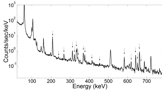
FIG. 2: Passive \gamma -ray spectrum of the ^{240}\text{Pu} target. The arrows indicate the 17 \gamma -ray peaks or multiplets used for determination of the target composition.
