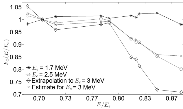
FIG. 4: The relative flux ratio, F_{\Phi}(E/E_e) , given in Eq. 3, was determined by comparing measured bremsstrahlung spectra at E_e = 1.7 and 2.5 MeV with MCNPX simulations of the measurements as functions of E/E_e . These values were extrapolated for E_e = 3.0 MeV (indicated by ‘ \diamond ’). Values representing half of the deviation from unity of the E_e = 3.0 MeV extrapolated values (indicated by ‘ \times ’) were used to scale the flux ratio in Eq. 2 and a corresponding systematic error, given in Table III, was assigned. The lines through the data points are guides to the eye.
