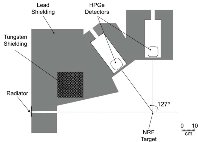
FIG. 1: Schematic of the experimental setup during active (beam-on) measurements. Additional Pb shielding was placed above and below the HPGe detectors (not shown).
