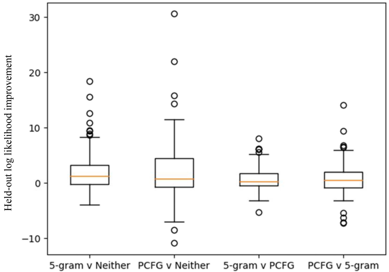
Figure 7: LANG likelihood improvement by participant.
