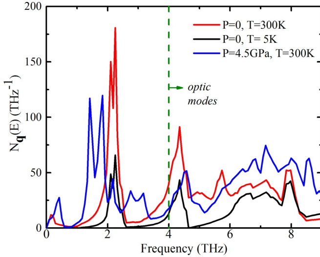
FIG. 4. N_q(E) vs frequency for T = 5\text{ K}, P = 0 (black curve), T = 300\text{ K}, P = 0 (red curve), and T = 300\text{ K}, P = 4.5\text{ GPa} (blue curve). Bose factors reduce N_q(E) for T = 5\text{ K} , thus the black curve is multiplied by five for better visibility. These curves correspond to q = (0.17, 0, 0.17) in units of 2\pi/a , where a is the lattice constant. Other randomly sampled q points give nearly identical behavior.
