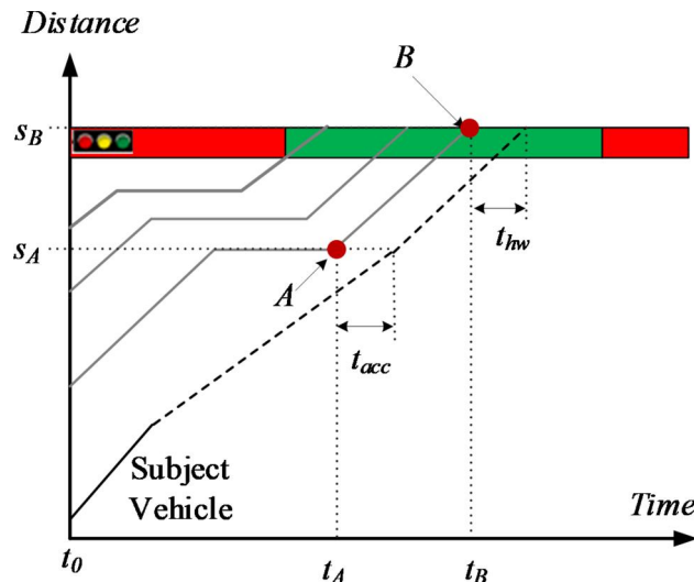
Figure 2. Position constraint for a subject CAV.
