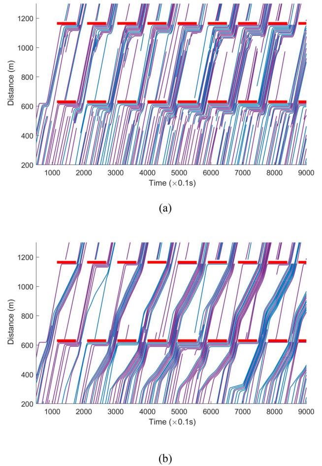
Figure 4. Vehicle trajectories in the baseline case (a) and EAD + LC + LT case (b). The purple curves depict MDV trajectories, and the blue curves depict CAV trajectories.
