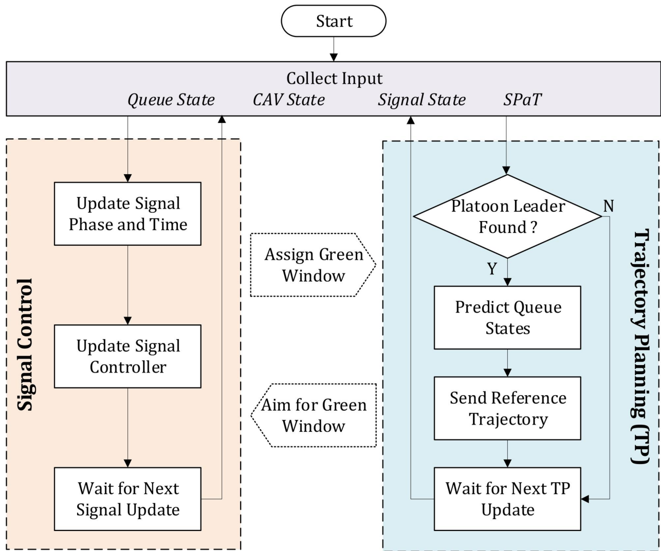
Figure 1. EAD control framework.
