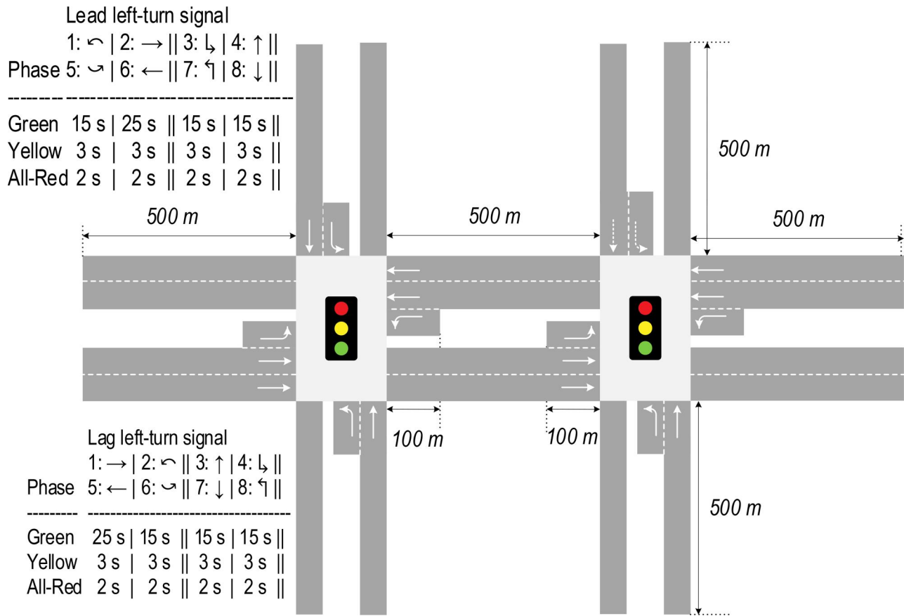
Figure 3. Study road network.
