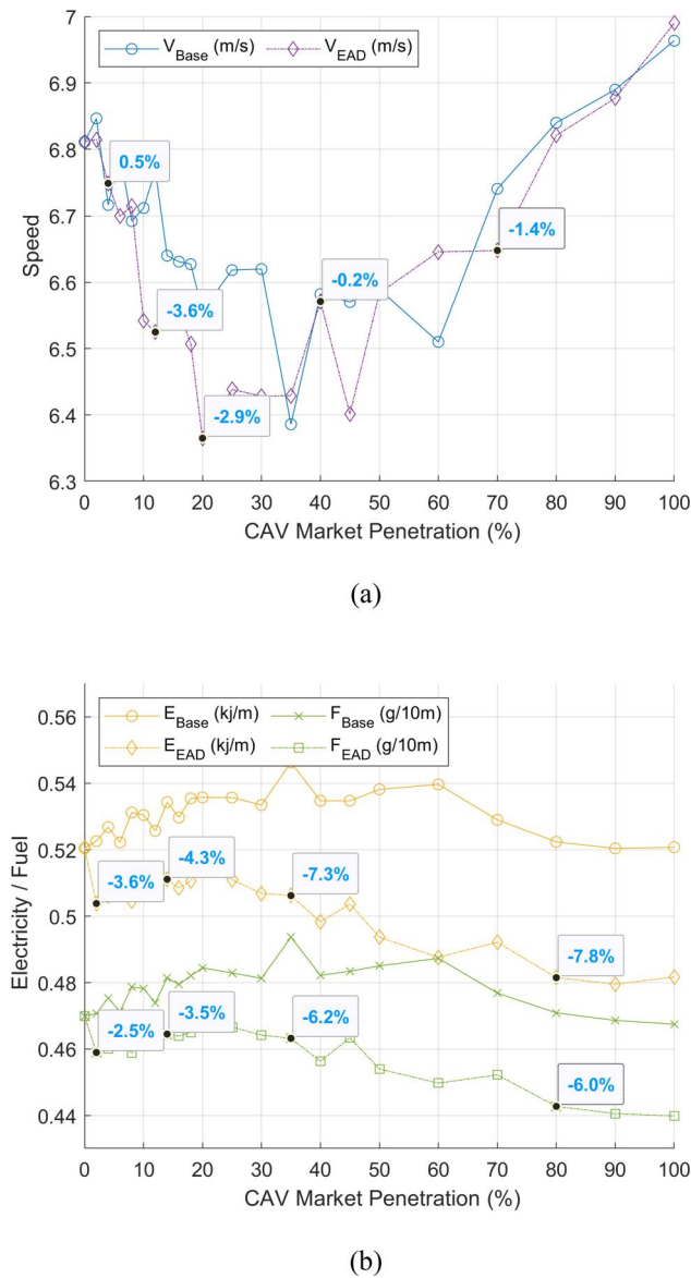
Figure 5. Average speed (a) and energy consumption (b) at different CAV MPR cases.
