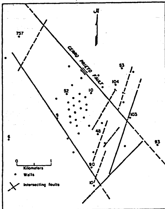
Figure 4: Location of known faults in the vicinity of the Cerro Prieto field, showing the intersecting faults and the location of wells and the very productive well No. 103.
