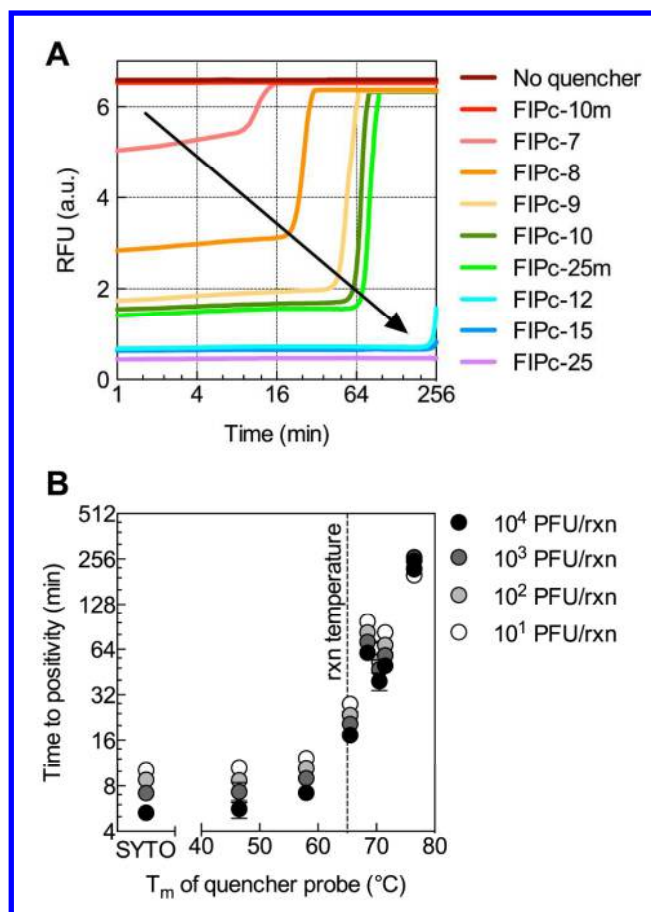
Figure 5. QUASR LAMP and DARQ LAMP exist on a continuum. A) Real-time fluorescence detection of 10,000 PFU equivalent WNV RNA per 10 \mu L reaction by RT-LAMP using FIP-ROX primer. Increasing the melting temperature of the FIP-complementary quencher probe decreases background fluorescence but dramatically slows amplification time. Quencher probes with internal base pair mismatches are denoted with the letter "m" at the end of their name. A full list of quencher probes is provided in Table S2. The arrow demonstrates the transition from QUASR RT-LAMP to DARQ RT-LAMP, represented by the full-length quenching probe FIPc-25. B) The time to positivity, determined by real time monitoring with SYTO dye in a separate fluorescence channel, increases dramatically as the FIP/FIPc complex melting temperature approaches and surpasses the reaction temperature for RT-LAMP. Melting temperature is far more important than even a 1,000-fold change in WNV template RNA concentration.
