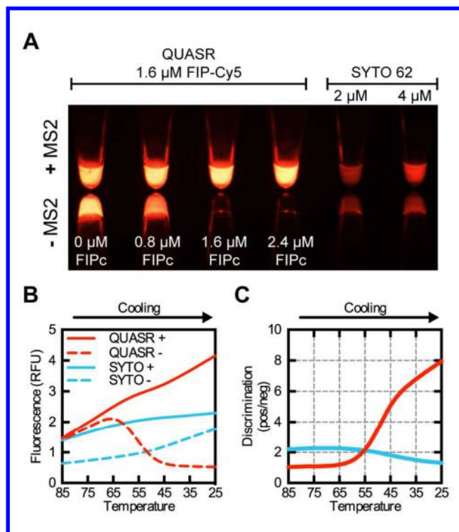
Figure 2. QUASR improves endpoint discrimination between positive and negative reactions compared to an intercalating dye. A) Comparison of room temperature endpoint detection with QUASR versus the intercalating dye SYTO 62 for RT-LAMP amplification of MS2 phage in PCR tubes. The top row of tubes shows positive reactions and the bottom row of tubes shows negative reactions. The 4 pairs of reactions on the left utilize QUASR via FIP-Cy5 with varying amounts of complementary quenching probe, FIPc, for detection. The 2 pairs of reactions on the right utilize SYTO 62 for detection. B) Annealing curves for QUASR (1.6 \mu M FIP-Cy5 with 2.4 \mu M FIPc) and SYTO 62 (4 \mu M) reactions post-amplification, by monitoring fluorescence in the Cy5 channel, while cooling from 85 ^{\circ} C to 25 ^{\circ} C in a real-time PCR machine. C) Signal discrimination (positive/negative fluorescence signal) as reactions cool from 85 ^{\circ} C to 25 ^{\circ} C.
