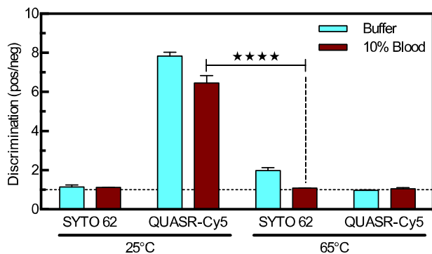
Figure 3. QUASR enables room temperature discrimination between positive and negative RT-LAMP reactions in 10% whole blood. In contrast, discrimination with SYTO 62 is completely lost in the presence of whole blood. Comparison by Tukey's test within 10% blood group following ANOVA, P < 0.0001 . Other differences were statistically significant but not shown.
