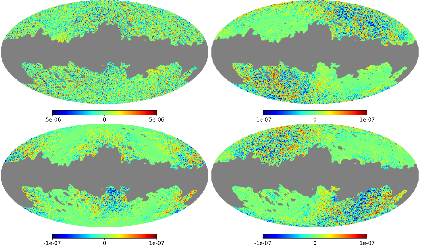
Fig. 1. Map of the tSZ effect from the MILCA component-separation method in y -map units (top left) and the expected modulated CMB signal (top right) generated using the SMICA-NQSZ CMB map in units of T_0 . The bottom left and right figures are the CMB anisotropies modulated in orthogonal directions to the CMB dipole, as explained in the text after Eq. (17). The greyed out region shows the mask used for our analysis. NILC and 2D-ILC y maps, as well as 2D-ILC CMB modulated anisotropies, are not shown, since they look essentially the same as the maps presented here. Note that the map of the tSZ effect (top left) has a different scale bar when compared to the other three (i.e., the modulation signal is about 50 times weaker).
