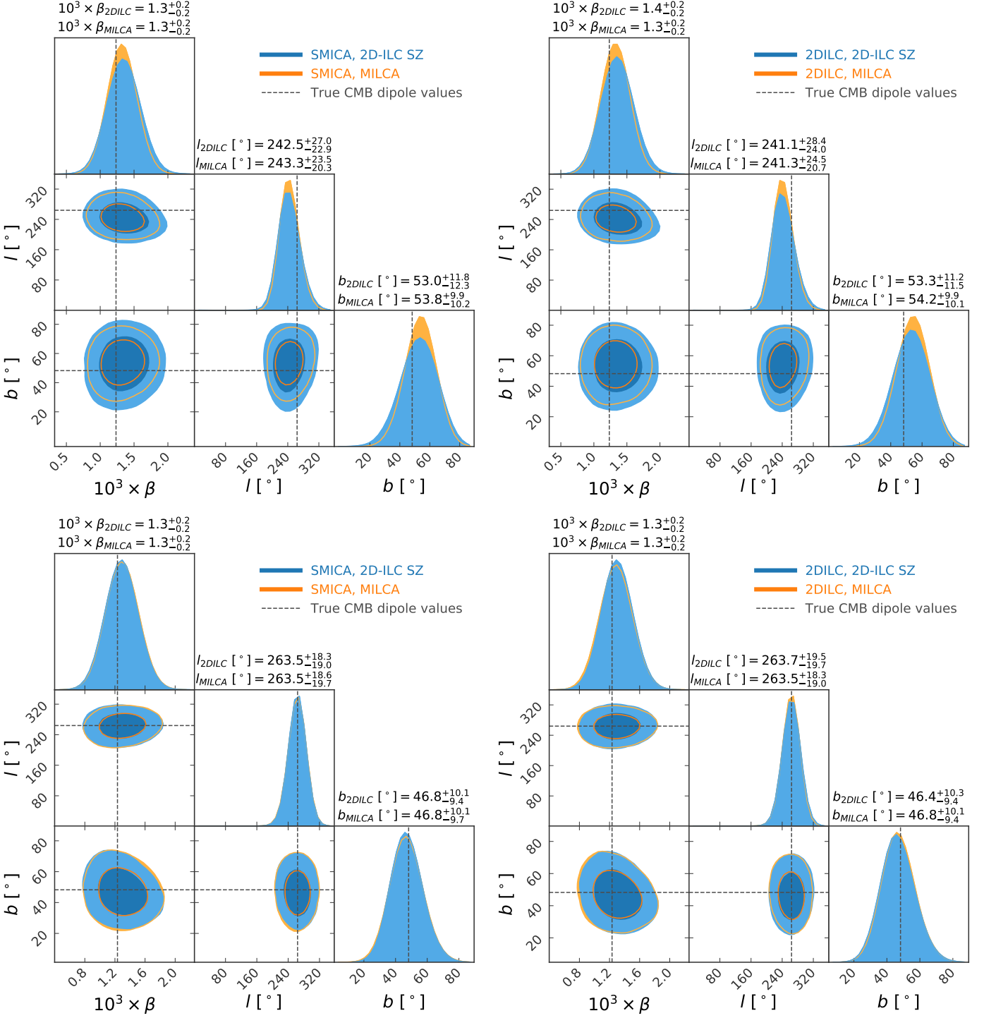
Fig. 2. Posteriors for the CMB dipole parameters using the map-space analysis (top) and harmonic-space analysis (bottom). The left panels use the SMICA-N0SZ CMB maps, whereas the right use the 2D-ILC CMB maps. MILCA y map results are shown in orange, and 2D-ILC y map results are shown in blue. Black dashed lines show the best-fit parameters from direct measurements of the CMB dipole. Dark and light contours enclose 68% and 95%, respectively. Titles for each panel give the best-fit results, along with the 68% uncertainties.
