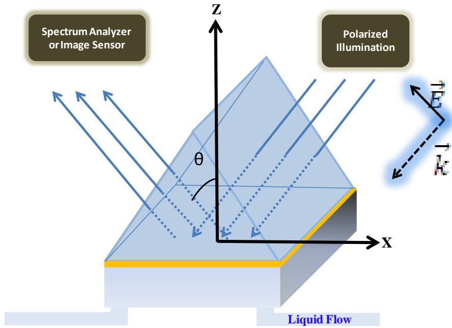
Figure 3-2 | The reflected light intensity in the total internal reflection condition is dependent on the total amount of biomolecules attached to the metal-dielectric interface, which can be used as a sensing tool for existing and quantifying biomolecules [26].
