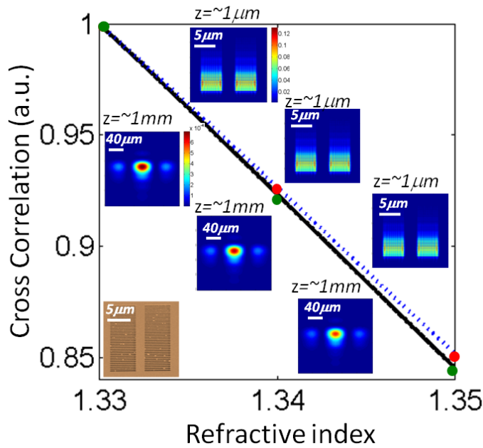
Figure 3-9 | Based on FDTD simulation results, the cross-correlation coefficients among lensfree transmission patterns of the same nanoaperture array shown in Figs. 3-4 are calculated as a function of the refractive index within the microchannel. These calculations were performed for both z \sim 1 \text{ mm} (solid line) and z \sim 1 \mu\text{m} (dotted line) planes. The false color insets depict the 2D transmission patterns for three different refractive index values (1.33, 1.34, and 1.35, respectively), where the upper (lower) ones are calculated at z \sim 1 \mu\text{m} ( z \sim 1 \text{ mm} ). Figure reprinted with permission from [48], copyright (2010), American Institute of Physics.
