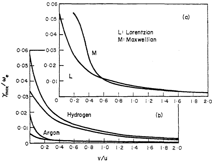
FIG. 2.—Growth rate of fastest growing wave (in units of \omega_e ) as a function of v/u . (a) comparison of collisionless results (for small T_i ) using Maxwellian (M) and Lorentzian (L) electron distributions in hydrogen. (b) effect of collisions on growth rate for hydrogen (upper 2 curves) and argon (lower 2 curves). For each species the upper curve is for \nu = 0 and the lower one for \nu = 0.2\omega_e .
