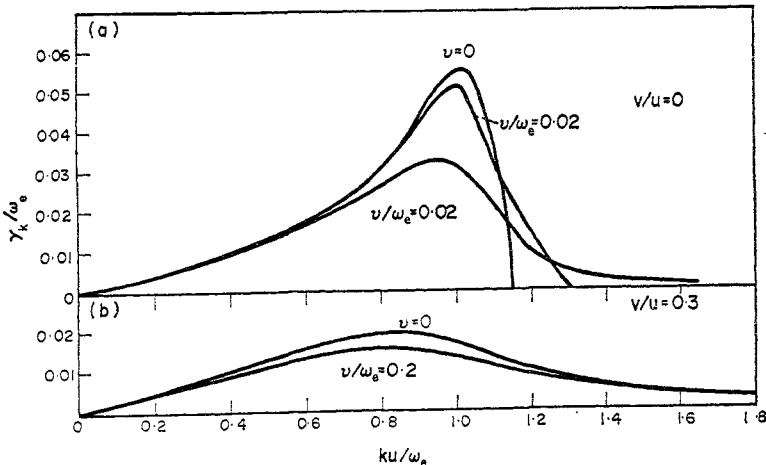
FIG. 1.—Growth rate \gamma_k vs. ku/\omega_e . (a) zero thermal spread. (b) v/u = 0.3 .
