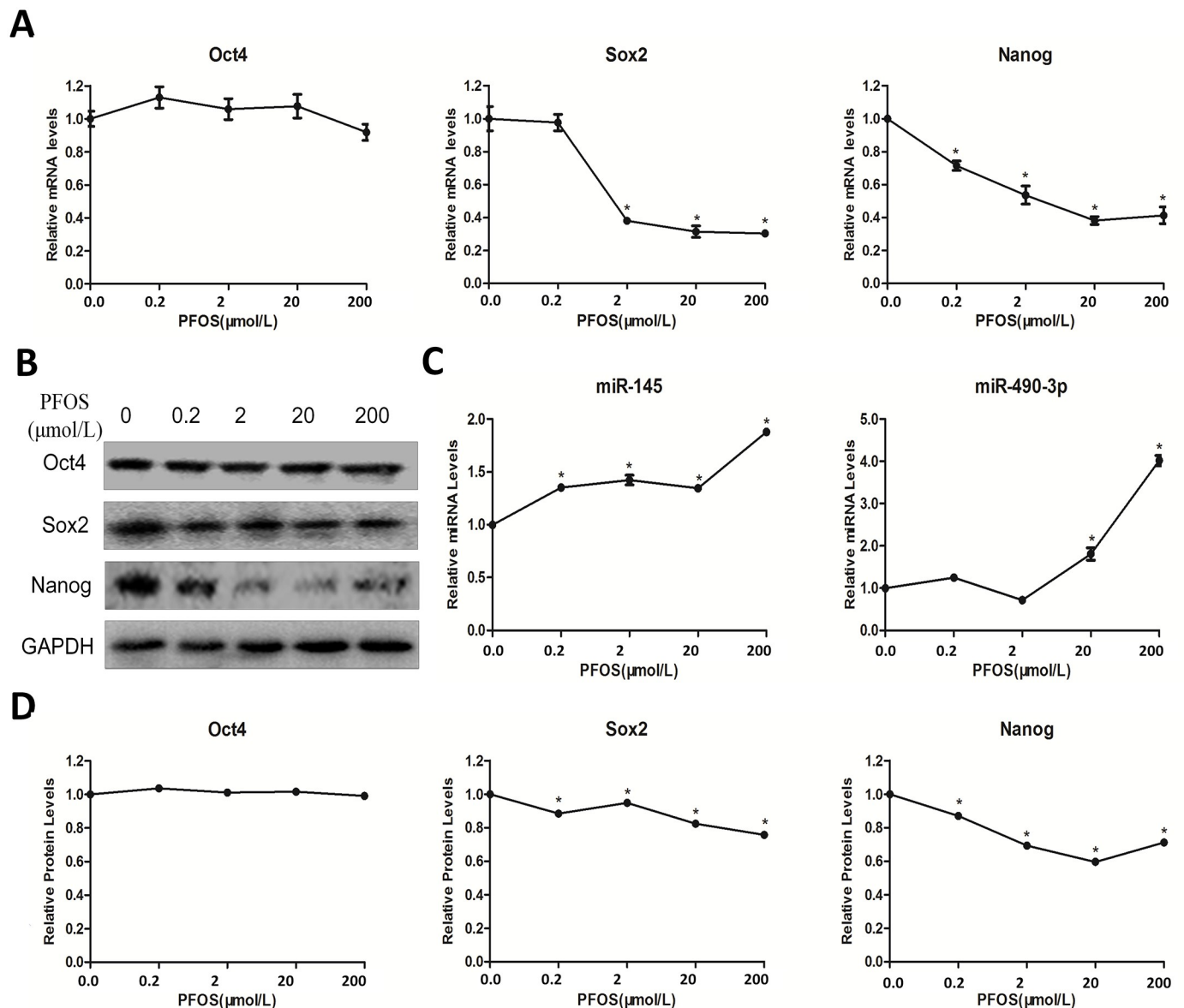
Fig 2. Effects of PFOS on pluripotency and expressions of miR-145 , miR-490-3p in mESCs. Cells were cultured with various concentrations of PFOS (0.2 \mu\text{M} , 2 \mu\text{M} , 20 \mu\text{M} , and 200 \mu\text{M} ) or DMSO as control for 24 h. (A) Oct-4/Sox-2/Nanog mRNA levels were determined by quantitative real-time PCR using a housekeeping gene GAPDH as an internal control. (B) The protein levels of Oct-4/Sox-2/Nanog were determined by Western blot analysis using GAPDH as an internal control. (C) miRNA levels ( miR-145 , miR-490-3p ) were determined by quantitative real-time PCR and were normalized to U6 as an internal control. Each data point was normalized to the control (DMSO) and represented the means \pm S.E. from three independent experiments. (D) Relative protein levels of Oct4, Sox2 and Nanog. * indicates significant difference when the values were compared to that of the control ( p < 0.05 ).
