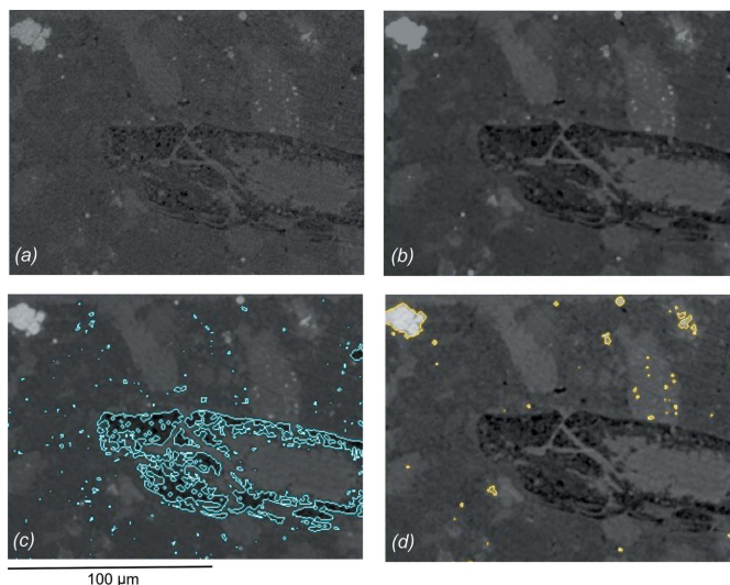
Figure 5 Images in the XY-plane of sample B1 obtained from the APS display an axial reconstructed slice (a) before and (b) after applying a 3D median filter, as well as the thresholding boundary of (c) low-density features and (d) pyrite.
