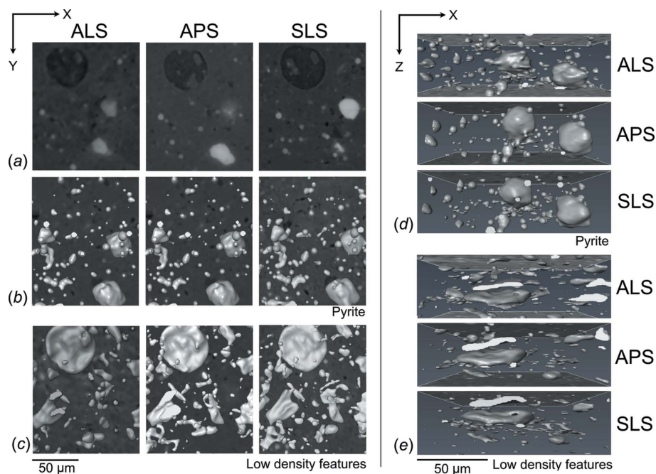
Figure 6 Images in the XY-plane show (a) axial slices through the cropped reconstructed volume of sample N1 after applying a 3D median filter, (b) the segmentation of pyrite, and (c) low-density features in 3D. Alternate views in the XZ-plane of the geometry and 3D distribution of (d) pyrite and (e) low-density features are also displayed.
