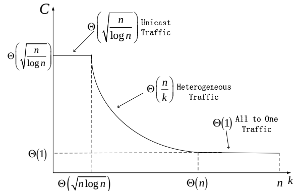
Fig. 4. The capacity result
