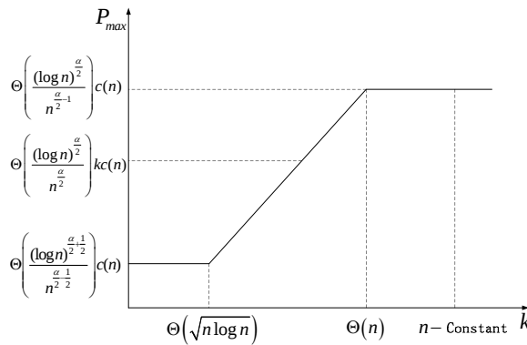
Fig. 5. The Growth of Power as a function of k
