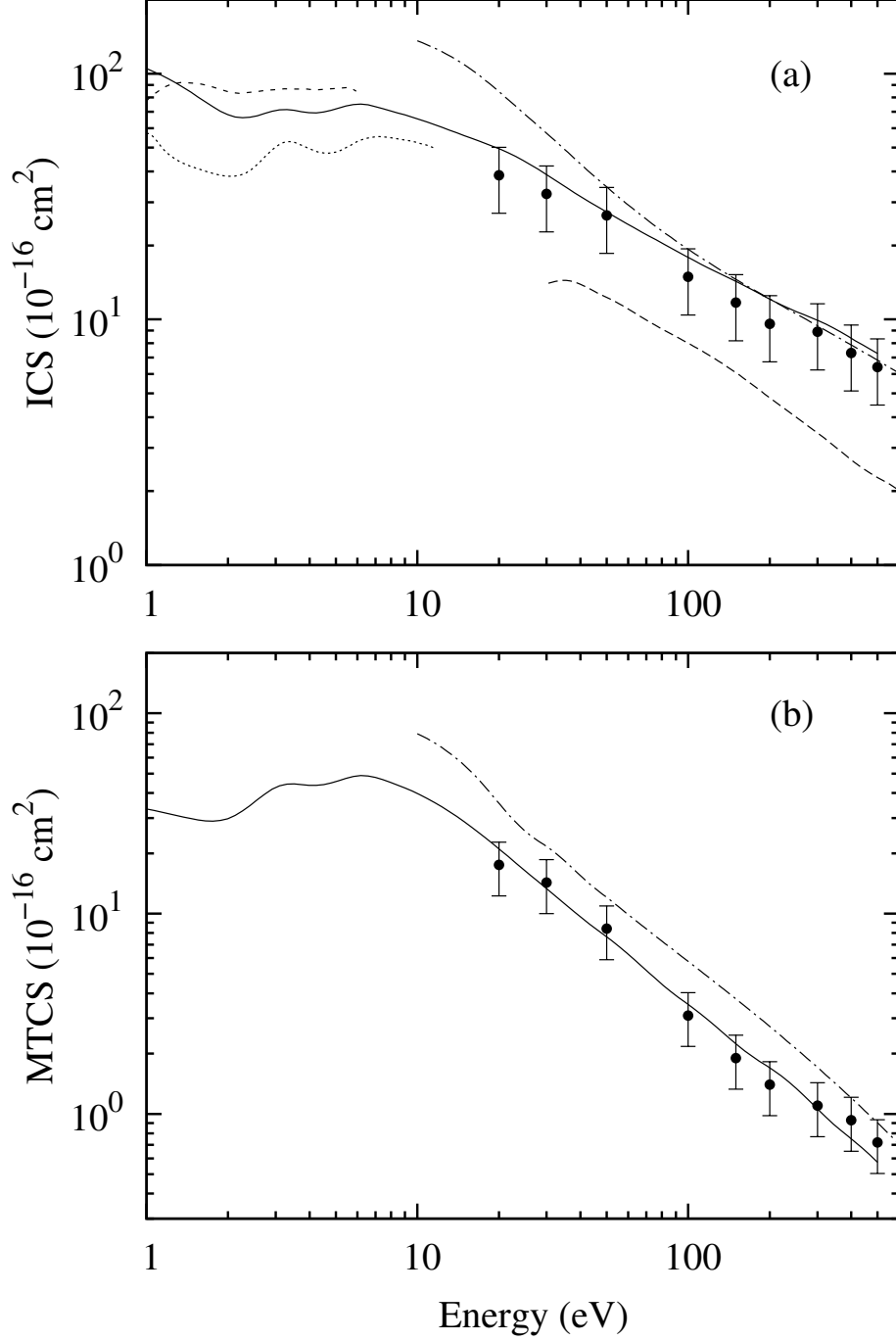
FIG. 5. (a) ICS and (b) MTCS for elastic e^- -dimethyl disulfide scattering. Full curve, present calculated data using the MCOP; dash-dotted curve, present calculated data using the IAM-AR; dashed curve, MSCOP ICS of Kaur et al. [6]; dotted curve, SMC ICS of Santos et al. [5]; short-dashed curve, ET spectrum of Dezarnaud-Dandine et al. [3] scaled by a factor of hundred; full circles, present experimental data.
