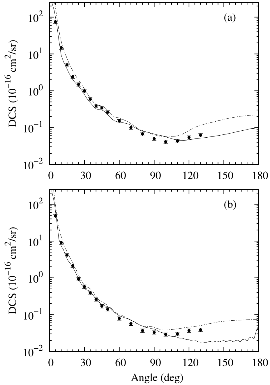
FIG. 4. Same as in Fig. 1 but at (a) 300 eV and (b) 500 eV.
