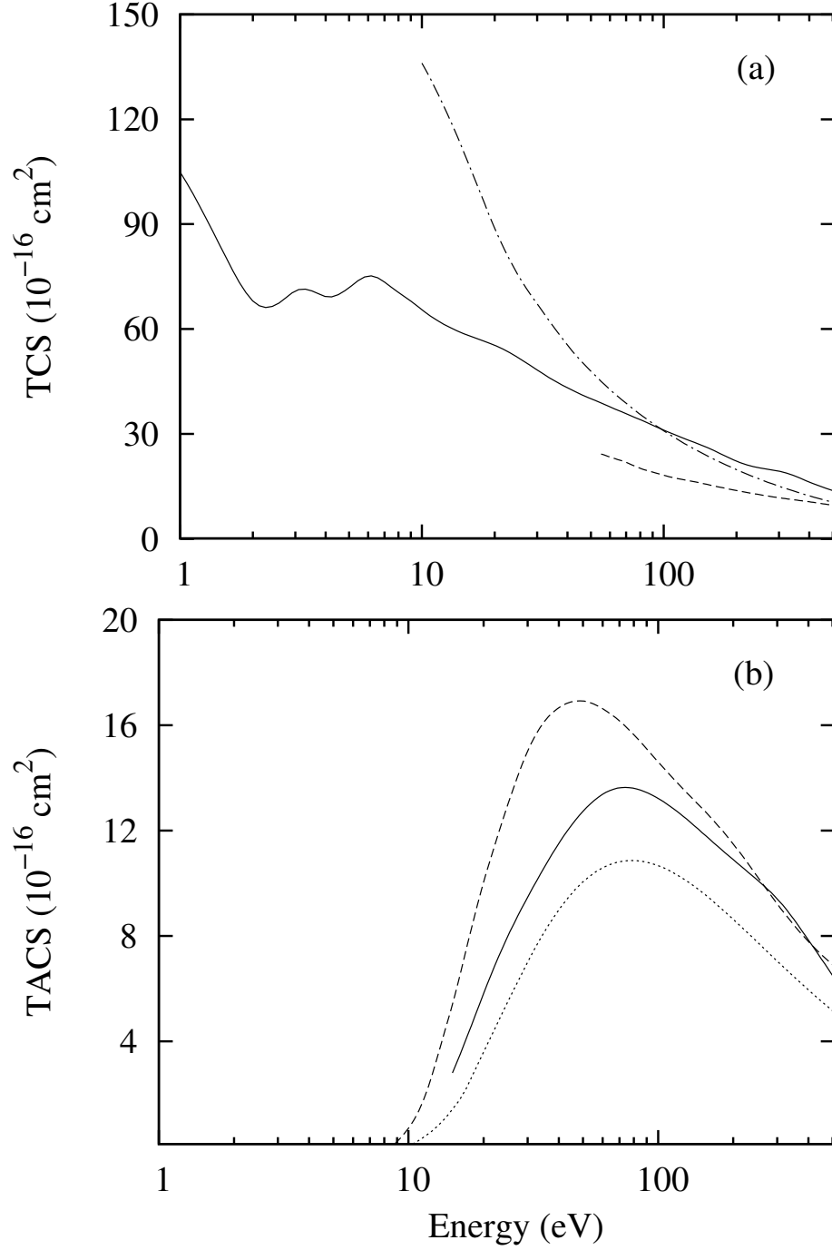
FIG. 6. (a) TCS and (b) TACS for e^- -dimethyl disulfide scattering. Full curve, present data calculated using the MCOP; dash-dotted curve, present calculated data using the IAM-AR; dashed curve, TCS and TICS of Kaur et al. calculated using the MSCOP [6]; dotted curve, present TICS calculated using BEB.
