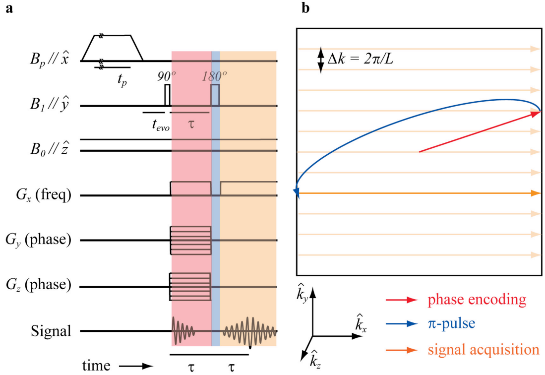
Figure 2.4: Pulse sequence for 2- and 3-d imaging. a. A standard ULF MRI imaging sequence. Sample magnetization is prepared by prepolarization with B_p for time t_p followed by relaxation in B_1 field for time t_{evo} to establish T_1 -contrast. Imaging consists of phase encoding (red), followed by a \pi -pulse (blue) and acquisition (orange). By varying the amplitude of the 1 (or two) phase encoding axes, k-space can be scanned in all three dimensions. b. x-y k-space plane. Phase encoding, \pi -pulse, and signal acquisition are shown as k-space trajectories. Coverage of k-space is shown as series of orange rays. The spacing of k-space lines scanned sets the field of view L = 2\pi/\Delta k , and the resolution \Delta l = \pi/k_{\max} is set by the maximum value of k-space scanned.
