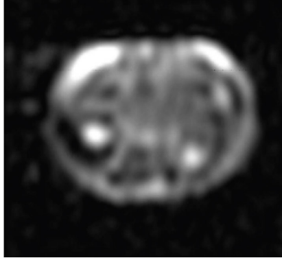
Figure 3.8: ULF MRI image of the human forearm, acquired with B_0 = 132 \mu\text{T} , B_p(\text{avg.}) = 40 \text{ mT} , and S_B^{1/2} = 1.5 \text{ fT Hz}^{-1/2} .
