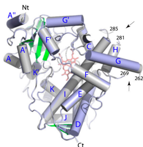
Figure 2. Superposition of two crystallographically independent molecules of CYP3A7. Molecules A and B and shown in gray and lavender, respectively. Helices and the N- and C-termini are labeled. The polypeptide breakage sites are indicated by arrows.
